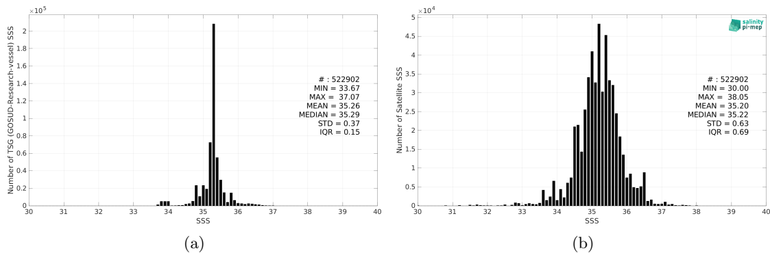
Figure 2: Histograms of SSS from TSG (GOSUD-Research-vessel) (a) and SMAP SSS L2 v5 (RSS) (b) considering all match-up pairs per bins of 0.1 over the Indian Ocean Pi-MEP region and for the full satellite product period.
