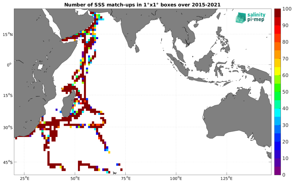
Figure 4: Number of SSS match-ups between TSG (GOSUD-Research-vessel) SSS and the SMAP SSS L2 v5 (RSS) SSS product for the Indian Ocean Pi-MEP region over 1^\circ \times 1^\circ boxes and for the full satellite product period.
