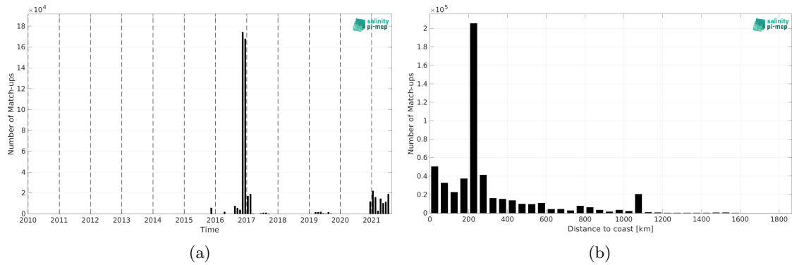
Figure 1: Number of match-ups between TSG (GOSUD-Research-vessel) and SMAP SSS L2 v5 (RSS) SSS as a function of time (a) and as function of the distance to coast (b) over the Indian Ocean Pi-MEP region and for the full satellite product period.
