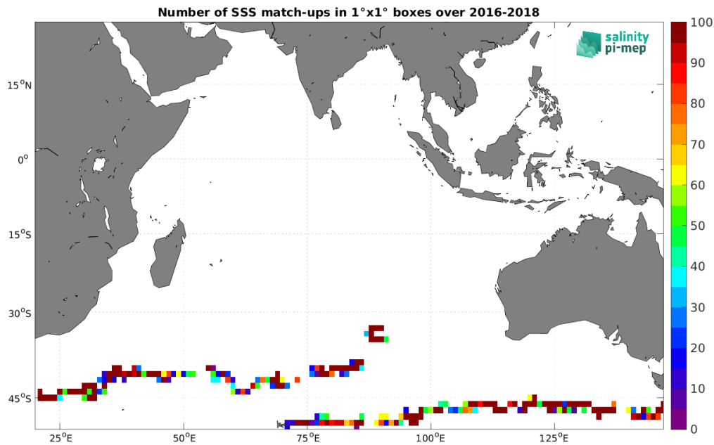
Figure 3: Number of SSS match-ups between Surface drifters SSS and the SMAP SSS L2 v5 (RSS) SSS product for the Indian Ocean Pi-MEP region over 1^\circ \times 1^\circ boxes and for the full satellite product period.
