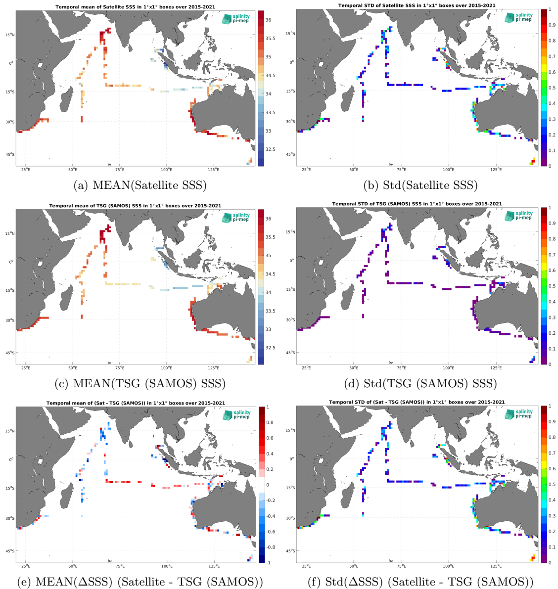
Figure 7: Temporal mean (left) and Std (right) of SSS from SMAP SSS L2 v5.3 (RSS) (top), TSG (SAMOS) (middle), and of \Delta SSS (Satellite - TSG (SAMOS)). Only match-up pairs are used to generate these maps.
