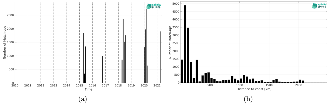
Figure 2: Number of match-ups between TSG (SAMOS) and SMAP SSS L2 v5.3 (RSS) SSS as a function of time (a) and as function of the distance to coast (b) over the Indian Ocean Pi-MEP region and for the full satellite product period.
