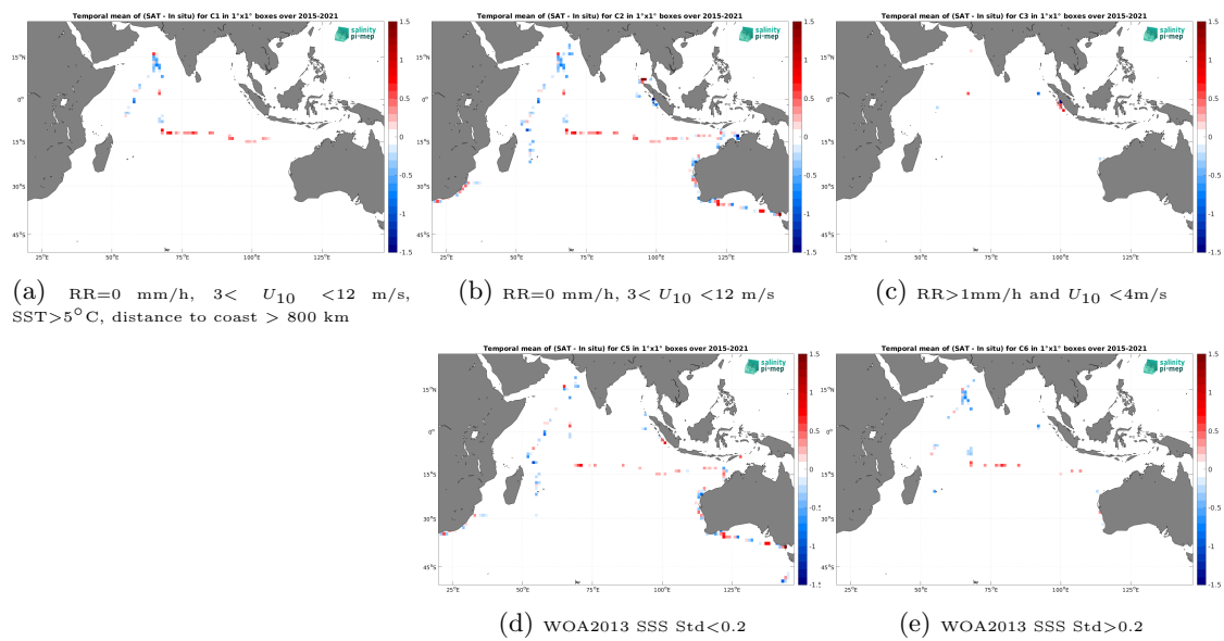
Figure 14: Temporal mean gridded over spatial boxes of size 1^\circ \times 1^\circ of \Delta SSS (SMAP SSS L2 v5.3 (RSS) - TSG (SAMOS)) for 5 different subdatasets corresponding to:RR=0 mm/h, 3 < U_{10} < 12 m/s, SST > 5^\circ\text{C} , distance to coast > 800 km (a), RR=0 mm/h, 3 < U_{10} < 12 m/s (b), RR > 1 mm/h and U_{10} < 4 m/s (c), WOA2013 SSS Std < 0.2 (d), WOA2013 SSS Std > 0.2 (e).
