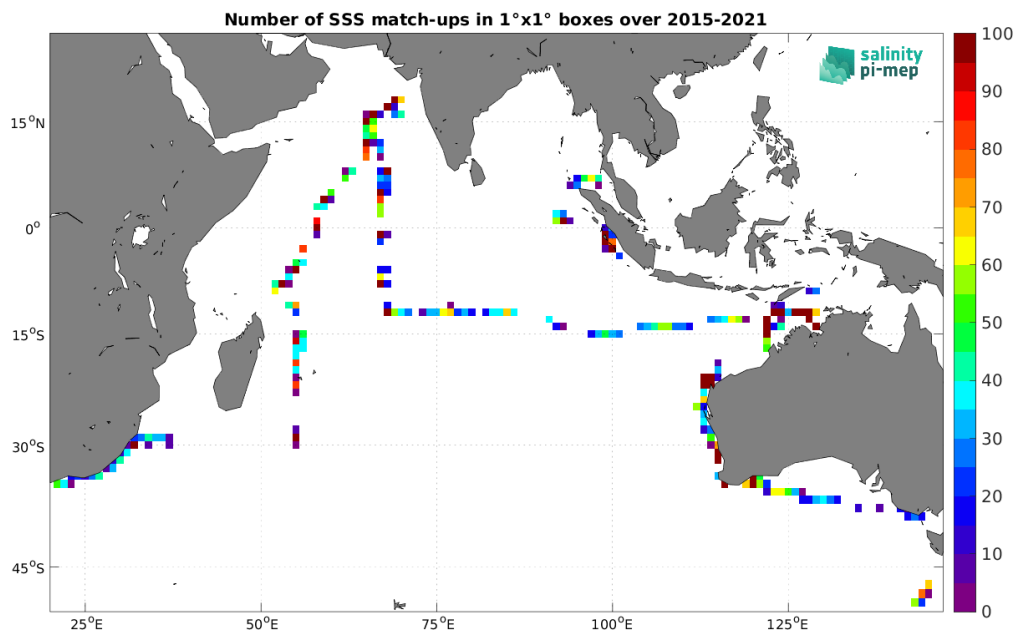
Figure 5: Number of SSS match-ups between TSG (SAMOS) SSS and the SMAP SSS L2 v5.3 (RSS) SSS product for the Indian Ocean Pi-MEP region over 1^\circ \times 1^\circ boxes and for the full satellite product period.
