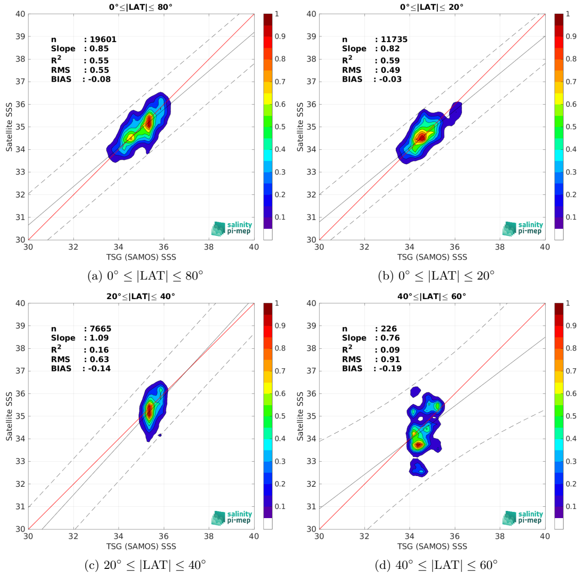
Figure 10: Contour maps of the concentration of SMAP SSS L2 v5.3 (RSS) SSS (y-axis) versus TSG (SAMOS) SSS (x-axis) at match-up pairs for different latitude bands. For each plot, the red line shows x=y . The black thin and dashed lines indicate a linear fit through the data cloud and the \pm 95\% confidence levels, respectively. The number match-up pairs n , the slope and R^2 coefficient of the linear fit, the root mean square (RMS) and the mean bias between satellite and in situ data are indicated for each latitude band in each plots.
