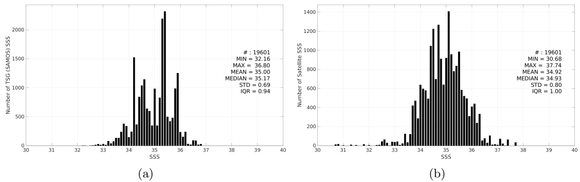
Figure 3: Histograms of SSS from TSG (SAMOS) (a) and SMAP SSS L2 v5.3 (RSS) (b) considering all match-up pairs per bins of 0.1 over the Indian Ocean Pi-MEP region and for the full satellite product period.
