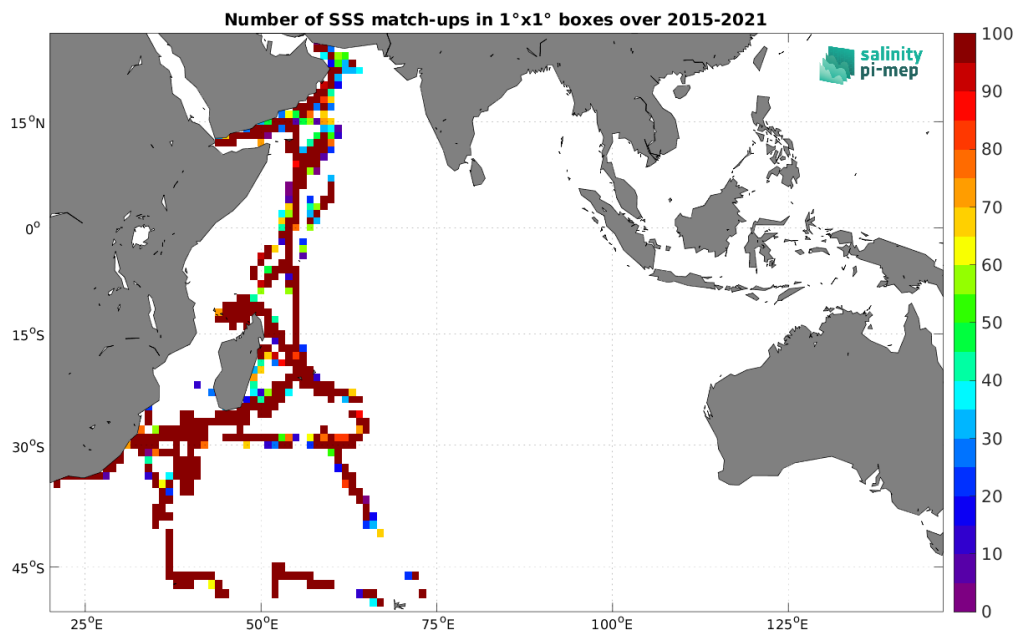
Figure 5: Number of SSS match-ups between TSG (GOSUD-Research-vessel) SSS and the SMAP SSS L2 v5.3 (RSS) SSS product for the Indian Ocean Pi-MEP region over 1^\circ \times 1^\circ boxes and for the full satellite product period.
