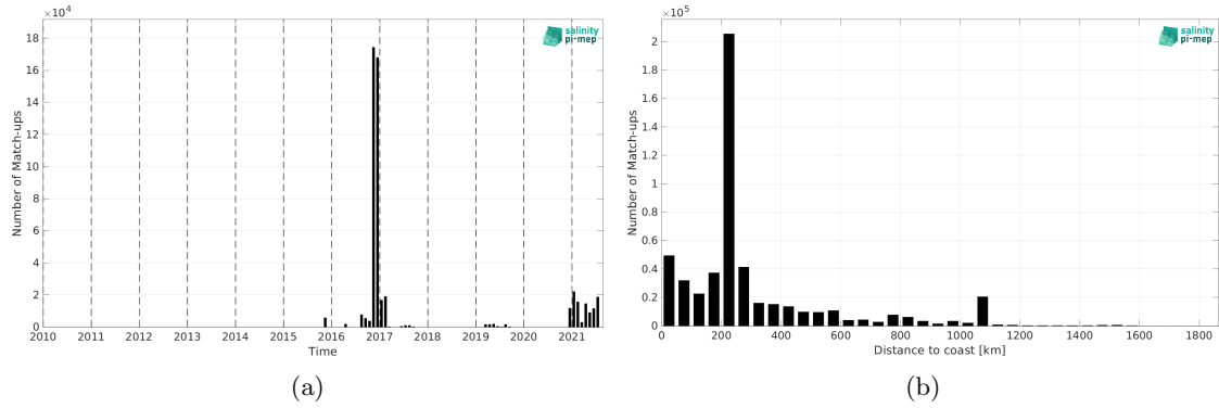
Figure 2: Number of match-ups between TSG (GOSUD-Research-vessel) and SMAP SSS L2 v5.3 (RSS) SSS as a function of time (a) and as function of the distance to coast (b) over the Indian Ocean Pi-MEP region and for the full satellite product period.
