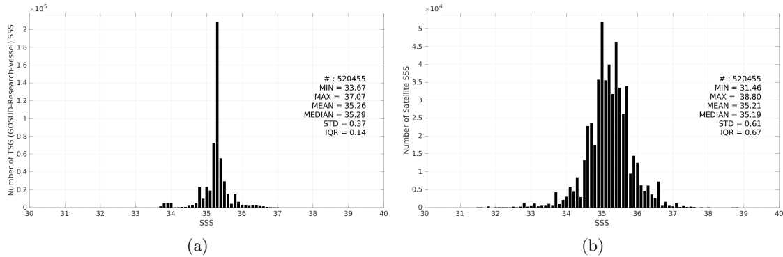
Figure 3: Histograms of SSS from TSG (GOSUD-Research-vessel) (a) and SMAP SSS L2 v5.3 (RSS) (b) considering all match-up pairs per bins of 0.1 over the Indian Ocean Pi-MEP region and for the full satellite product period.
