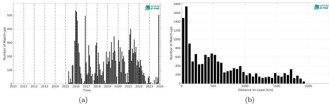
Figure 2: Number of match-ups between Marine mammals and SMAP SSS L2 v5.3 (RSS) SSS as a function of time (a) and as function of the distance to coast (b) over the Indian Ocean Pi-MEP region and for the full satellite product period.
