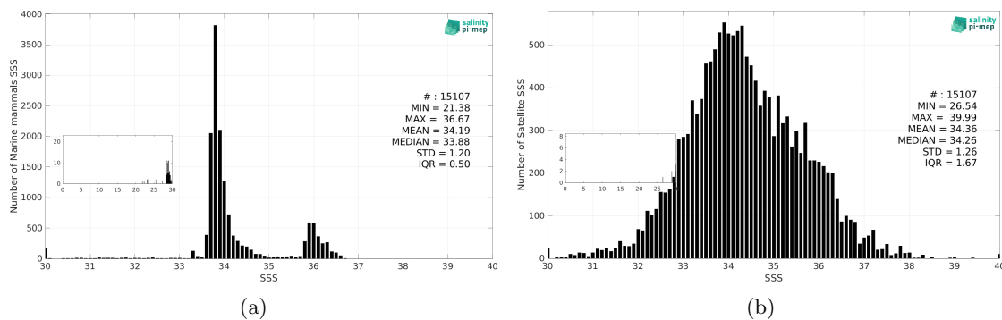
Figure 3: Histograms of SSS from Marine mammals (a) and SMAP SSS L2 v5.3 (RSS) (b) considering all match-up pairs per bins of 0.1 over the Indian Ocean Pi-MEP region and for the full satellite product period.
