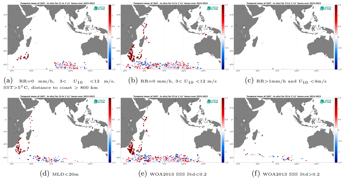
Figure 14: Temporal mean gridded over spatial boxes of size 1^\circ \times 1^\circ of \Delta\text{SSS} (SMAP SSS L2 v5.3 (RSS) - Marine mammals) for 6 different subdatasets corresponding to:RR=0 mm/h, 3 < U_{10} < 12 m/s, SST>5°C, distance to coast > 800 km (a), RR=0 mm/h, 3 < U_{10} < 12 m/s (b), RR>1mm/h and U_{10} < 4 m/s (c),MLD<20m (d),WOA2013 SSS Std<0.2 (e),WOA2013 SSS Std>0.2 (f).
