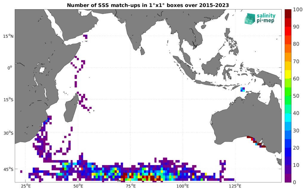
Figure 5: Number of SSS match-ups between Marine mammals SSS and the SMAP SSS L2 v5.3 (RSS) SSS product for the Indian Ocean Pi-MEP region over 1^\circ \times 1^\circ boxes and for the full satellite product period.
