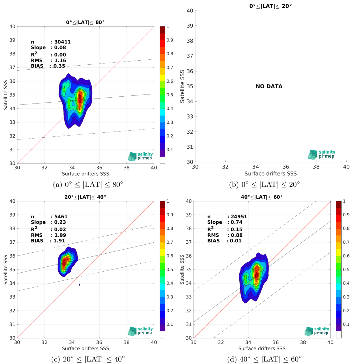
Figure 9: Contour maps of the concentration of SMAP SSS L2 v5.3 (RSS) SSS (y-axis) versus Surface drifters SSS (x-axis) at match-up pairs for different latitude bands. For each plot, the red line shows x=y . The black thin and dashed lines indicate a linear fit through the data cloud and the \pm 95\% confidence levels, respectively. The number match-up pairs n , the slope and R^2 coefficient of the linear fit, the root mean square (RMS) and the mean bias between satellite and in situ data are indicated for each latitude band in each plots.
