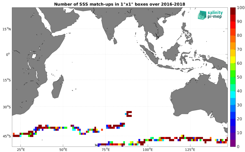
Figure 4: Number of SSS match-ups between Surface drifters SSS and the SMAP SSS L2 v5.3 (RSS) SSS product for the Indian Ocean Pi-MEP region over 1^\circ \times 1^\circ boxes and for the full satellite product period.
