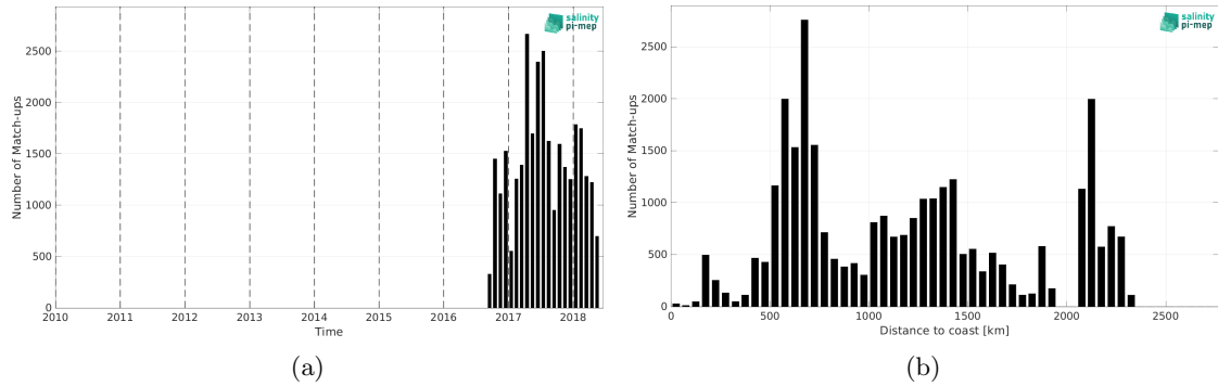
Figure 2: Number of match-ups between Surface drifters and SMAP SSS L2 v5.3 (RSS) SSS as a function of time (a) and as function of the distance to coast (b) over the Indian Ocean Pi-MEP region and for the full satellite product period.
