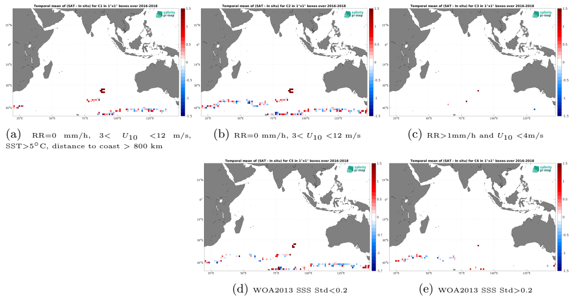
Figure 13: Temporal mean gridded over spatial boxes of size 1^\circ \times 1^\circ of \Delta SSS (SMAP SSS L2 v5.3 (RSS) - Surface drifters) for 5 different subdatasets corresponding to:RR=0 mm/h, 3 < U_{10} < 12 m/s, SST >5^\circ\text{C} , distance to coast > 800 km (a), RR=0 mm/h, 3 < U_{10} < 12 m/s (b), RR >1 mm/h and U_{10} < 4 m/s (c), WOA2013 SSS Std <0.2 (d), WOA2013 SSS Std >0.2 (e).
