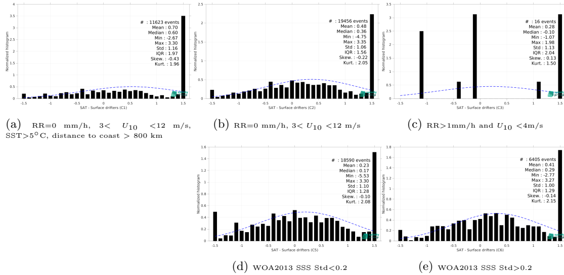
Figure 14: Normalized histogram of \Delta SSS (SMAP SSS L2 v5.3 (RSS) - Surface drifters) for 5 different subdatasets corresponding to: RR=0 mm/h, 3 < U_{10} < 12 m/s, SST > 5°C, distance to coast > 800 km (a), RR=0 mm/h, 3 < U_{10} < 12 m/s (b), RR > 1mm/h and U_{10} < 4 m/s (c), WOA2013 SSS Std < 0.2 (d), WOA2013 SSS Std > 0.2 (e).
