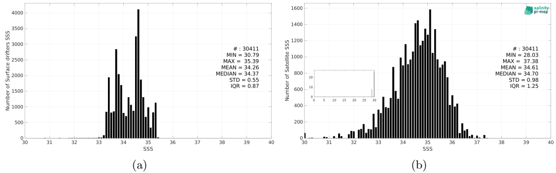
Figure 3: Histograms of SSS from Surface drifters (a) and SMAP SSS L2 v5.3 (RSS) (b) considering all match-up pairs per bins of 0.1 over the Indian Ocean Pi-MEP region and for the full satellite product period.
