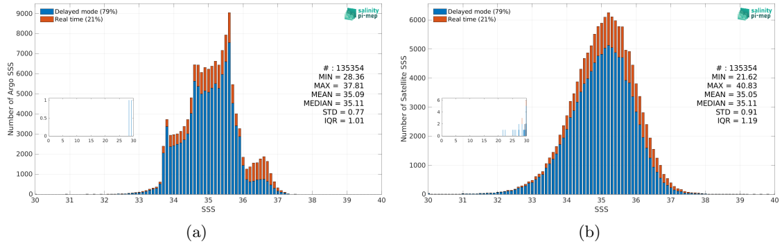
Figure 3: Histograms of SSS from Argo (a) and SMAP SSS L2 v5.3 (RSS) (b) considering all match-up pairs per bins of 0.1 over the Indian Ocean Pi-MEP region and for the full satellite product period.
