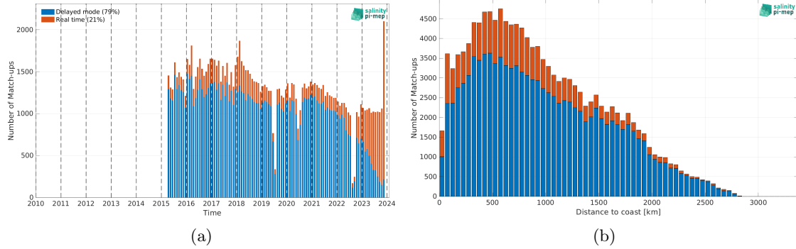
Figure 2: Number of match-ups between Argo and SMAP SSS L2 v5.3 (RSS) SSS as a function of time (a) and as function of the distance to coast (b) over the Indian Ocean Pi-MEP region and for the full satellite product period.
