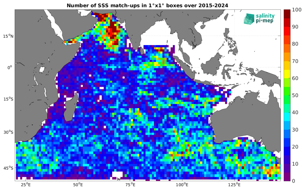
Figure 5: Number of SSS match-ups between Argo SSS and the SMAP SSS L2 v5.3 (RSS) SSS product for the Indian Ocean Pi-MEP region over 1^\circ \times 1^\circ boxes and for the full satellite product period.
