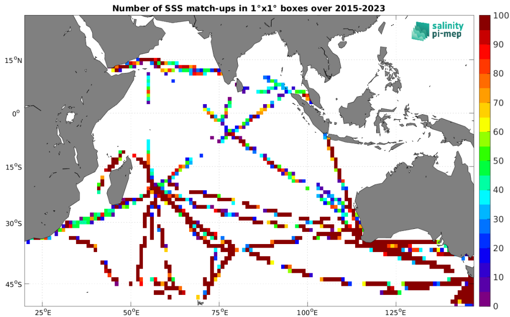
Figure 5: Number of SSS match-ups between TSG (LEGOS-DM) SSS and the SMAP SSS L2 v5.3 - 40 km (RSS) SSS product for the Indian Ocean Pi-MEP region over 1^\circ \times 1^\circ boxes and for the full satellite product period.
