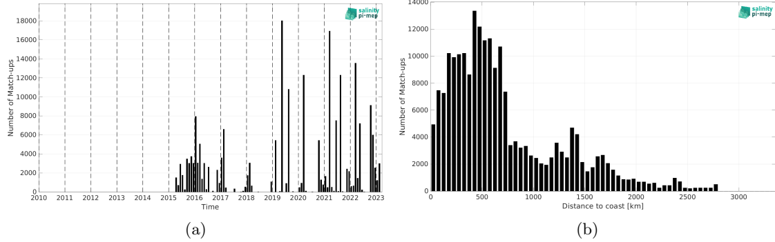
Figure 2: Number of match-ups between TSG (LEGOS-DM) and SMAP SSS L2 v5.3 - 40 km (RSS) SSS as a function of time (a) and as function of the distance to coast (b) over the Indian Ocean Pi-MEP region and for the full satellite product period.
