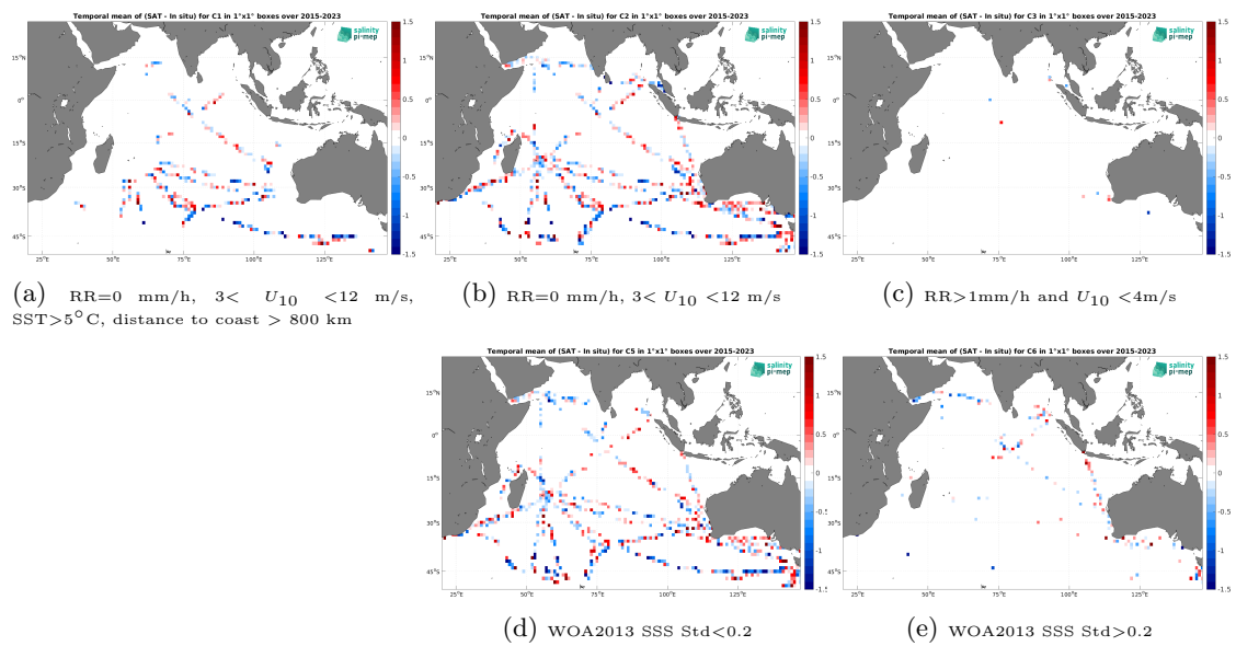
Figure 14: Temporal mean gridded over spatial boxes of size 1^\circ \times 1^\circ of \Delta SSS (SMAP SSS L2 v5.3 - 40 km (RSS) - TSG (LEGOS-DM)) for 5 different subdatasets corresponding to:RR=0 mm/h, 3 < U_{10} < 12 m/s, SST > 5^\circ\text{C} , distance to coast > 800 km (a), RR=0 mm/h, 3 < U_{10} < 12 m/s (b), RR > 1 mm/h and U_{10} < 4 m/s (c), WOA2013 SSS Std < 0.2 (d), WOA2013 SSS Std > 0.2 (e).
