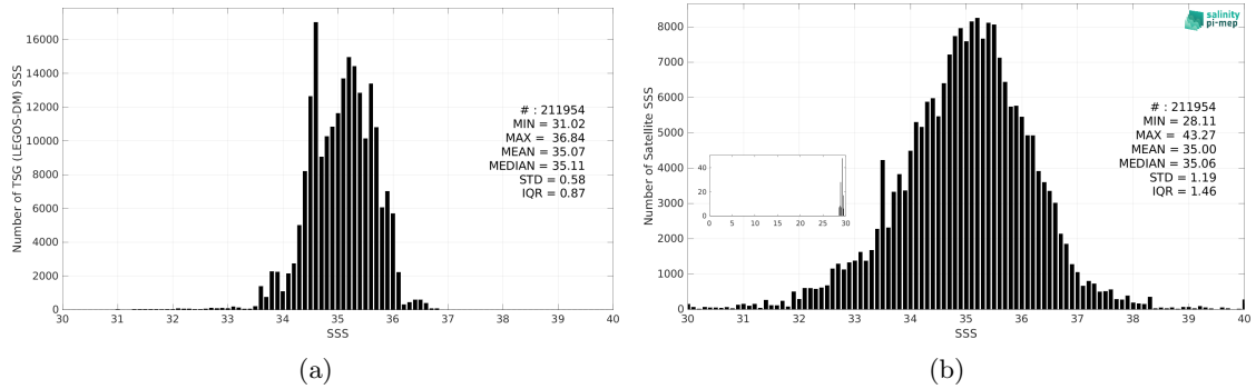
Figure 3: Histograms of SSS from TSG (LEGOS-DM) (a) and SMAP SSS L2 v5.3 - 40 km (RSS) (b) considering all match-up pairs per bins of 0.1 over the Indian Ocean Pi-MEP region and for the full satellite product period.
