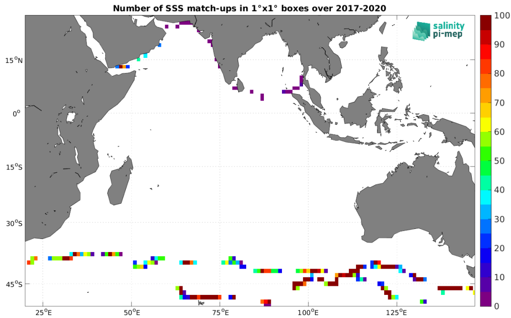
Figure 5: Number of SSS match-ups between TSG (GOSUD-Sailing-ship) SSS and the SMAP SSS L2 v5.3 - 40 km (RSS) SSS product for the Indian Ocean Pi-MEP region over 1^\circ \times 1^\circ boxes and for the full satellite product period.
