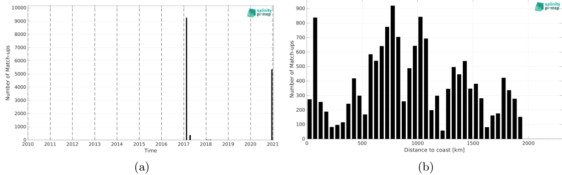
Figure 2: Number of match-ups between TSG (GOSUD-Sailing-ship) and SMAP SSS L2 v5.3 - 40 km (RSS) SSS as a function of time (a) and as function of the distance to coast (b) over the Indian Ocean Pi-MEP region and for the full satellite product period.
