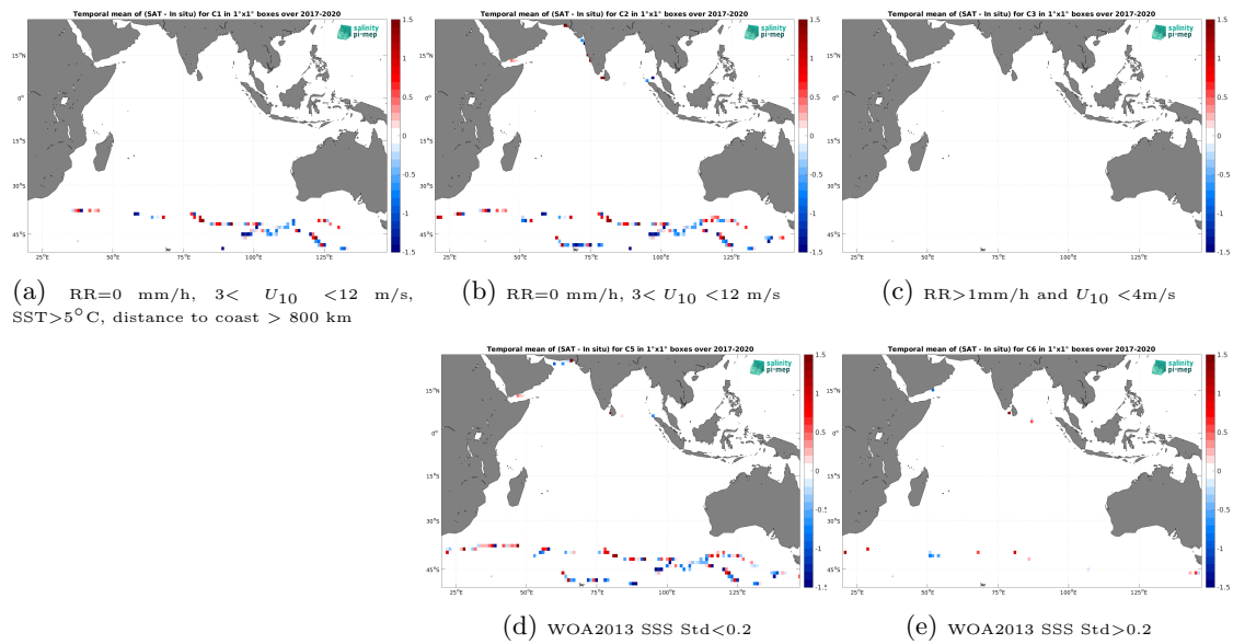
Figure 14: Temporal mean gridded over spatial boxes of size 1^\circ \times 1^\circ of \Delta SSS (SMAP SSS L2 v5.3 - 40 km (RSS) - TSG (GOSUD-Sailing-ship)) for 5 different subdatasets corresponding to:RR=0 mm/h, 3 < U_{10} < 12 m/s, SST >5^\circ C, distance to coast > 800 km (a), RR=0 mm/h, 3 < U_{10} < 12 m/s (b), RR >1 mm/h and U_{10} < 4 m/s (c), WOA2013 SSS Std <0.2 (d), WOA2013 SSS Std >0.2 (e).
