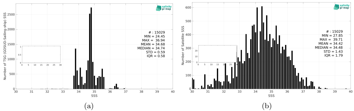
Figure 3: Histograms of SSS from TSG (GOSUD-Sailing-ship) (a) and SMAP SSS L2 v5.3 - 40 km (RSS) (b) considering all match-up pairs per bins of 0.1 over the Indian Ocean Pi-MEP region and for the full satellite product period.
