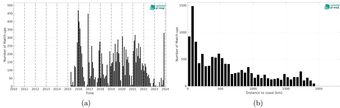
Figure 2: Number of match-ups between Marine mammals and SMAP SSS L2 v5.3 - 40 km (RSS) SSS as a function of time (a) and as function of the distance to coast (b) over the Indian Ocean Pi-MEP region and for the full satellite product period.
