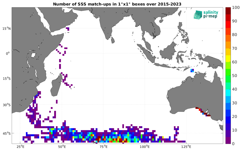
Figure 5: Number of SSS match-ups between Marine mammals SSS and the SMAP SSS L2 v5.3 - 40 km (RSS) SSS product for the Indian Ocean Pi-MEP region over 1^\circ \times 1^\circ boxes and for the full satellite product period.
