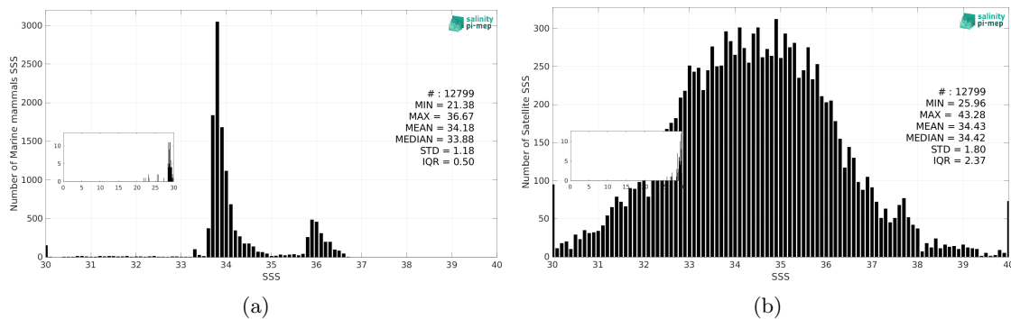
Figure 3: Histograms of SSS from Marine mammals (a) and SMAP SSS L2 v5.3 - 40 km (RSS) (b) considering all match-up pairs per bins of 0.1 over the Indian Ocean Pi-MEP region and for the full satellite product period.
