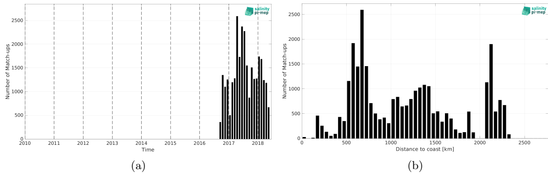
Figure 2: Number of match-ups between Surface drifters and SMAP SSS L2 v5.3 - 40 km (RSS) SSS as a function of time (a) and as function of the distance to coast (b) over the Indian Ocean Pi-MEP region and for the full satellite product period.
