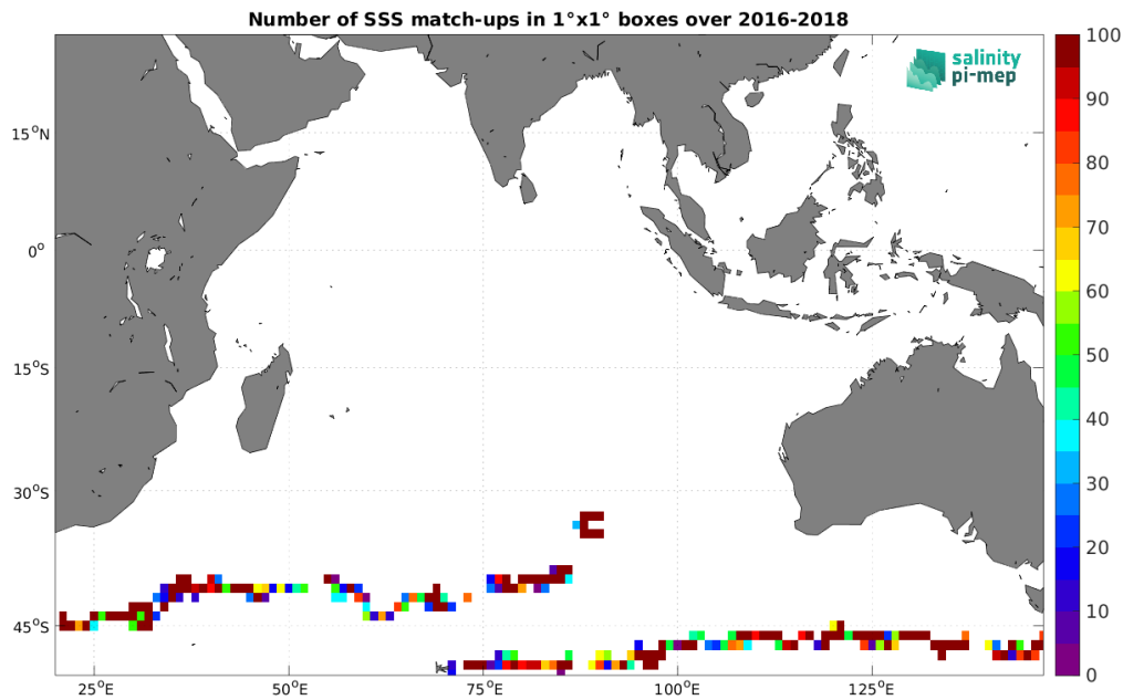
Figure 4: Number of SSS match-ups between Surface drifters SSS and the SMAP SSS L2 v5.3 - 40 km (RSS) SSS product for the Indian Ocean Pi-MEP region over 1^\circ \times 1^\circ boxes and for the full satellite product period.
