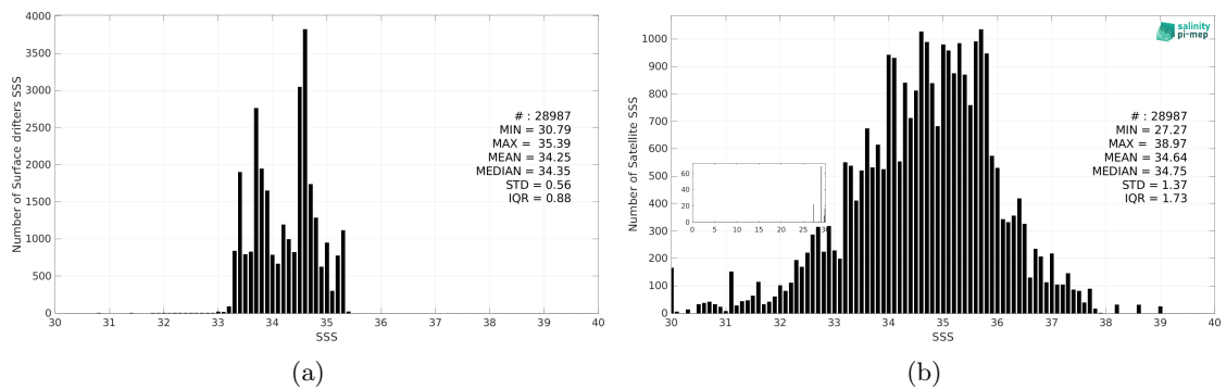
Figure 3: Histograms of SSS from Surface drifters (a) and SMAP SSS L2 v5.3 - 40 km (RSS) (b) considering all match-up pairs per bins of 0.1 over the Indian Ocean Pi-MEP region and for the full satellite product period.
