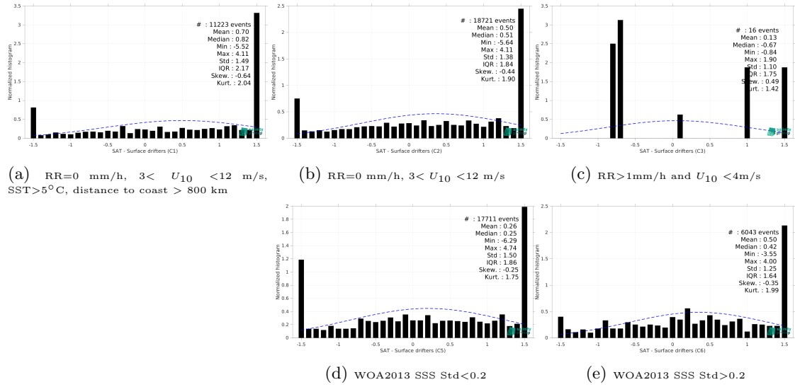
Figure 14: Normalized histogram of \Delta SSS (SMAP SSS L2 v5.3 - 40 km (RSS) - Surface drifters) for 5 different subdatasets corresponding to: RR=0 mm/h, 3 < U_{10} < 12 m/s, SST>5°C, distance to coast > 800 km (a), RR=0 mm/h, 3 < U_{10} < 12 m/s (b), RR>1mm/h and U_{10} < 4 m/s (c), WOA2013 SSS Std<0.2 (d), WOA2013 SSS Std>0.2 (e).
