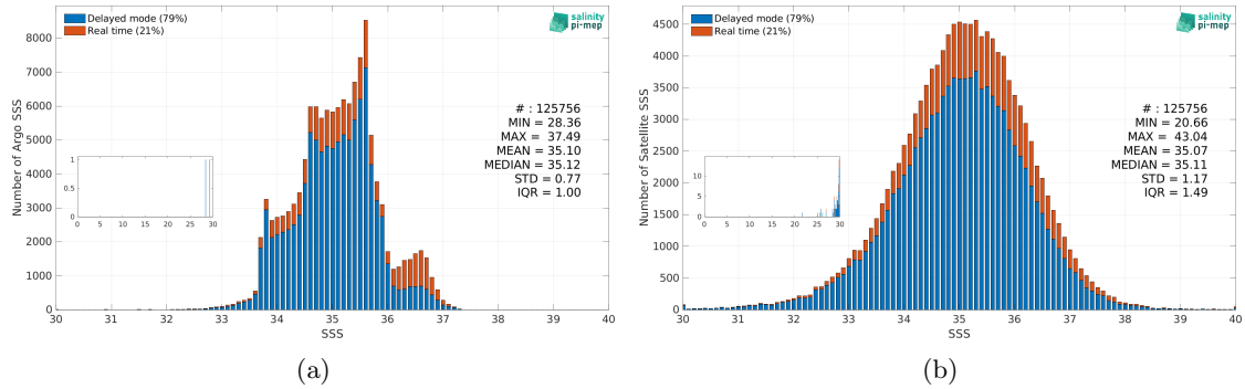
Figure 3: Histograms of SSS from Argo (a) and SMAP SSS L2 v5.3 - 40 km (RSS) (b) considering all match-up pairs per bins of 0.1 over the Indian Ocean Pi-MEP region and for the full satellite product period.
