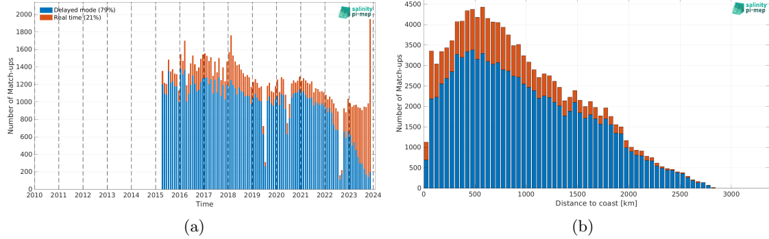
Figure 2: Number of match-ups between Argo and SMAP SSS L2 v5.3 - 40 km (RSS) SSS as a function of time (a) and as function of the distance to coast (b) over the Indian Ocean Pi-MEP region and for the full satellite product period.
