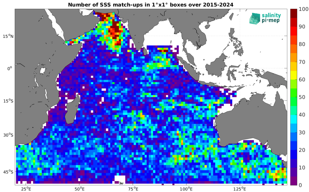
Figure 5: Number of SSS match-ups between Argo SSS and the SMAP SSS L2 v5.3 - 40 km (RSS) SSS product for the Indian Ocean Pi-MEP region over 1^\circ \times 1^\circ boxes and for the full satellite product period.
