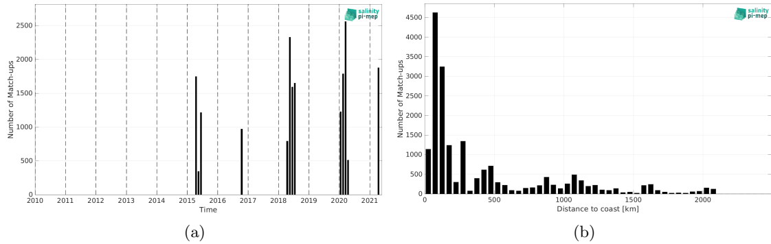
Figure 1: Number of match-ups between TSG (SAMOS) and SMAP SSS L2 v5 - 40 km (RSS) SSS as a function of time (a) and as function of the distance to coast (b) over the Indian Ocean Pi-MEP region and for the full satellite product period.
