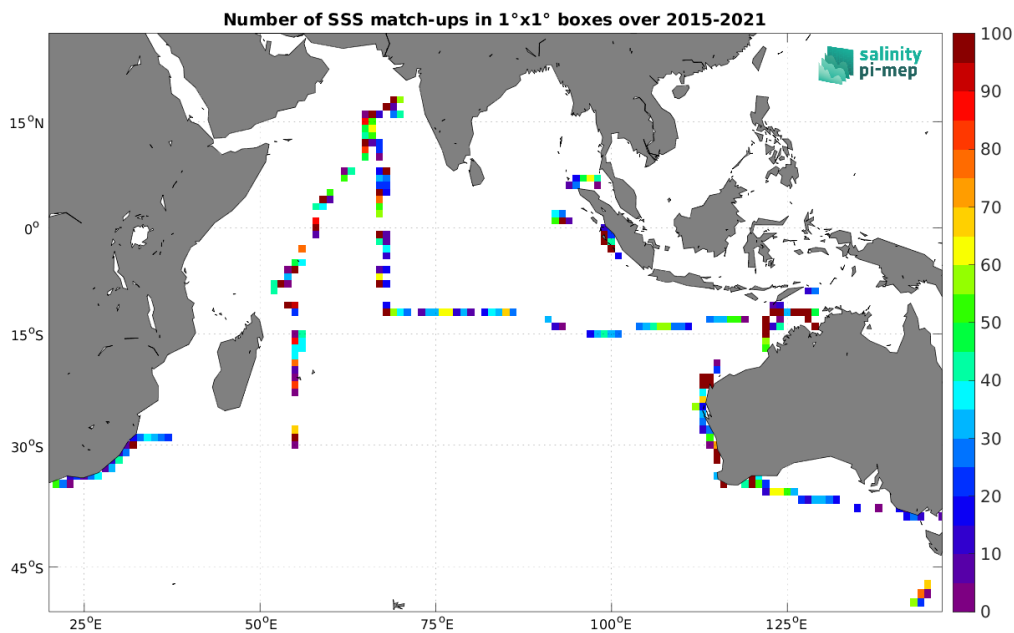
Figure 4: Number of SSS match-ups between TSG (SAMOS) SSS and the SMAP SSS L2 v5 - 40 km (RSS) SSS product for the Indian Ocean Pi-MEP region over 1^\circ \times 1^\circ boxes and for the full satellite product period.
