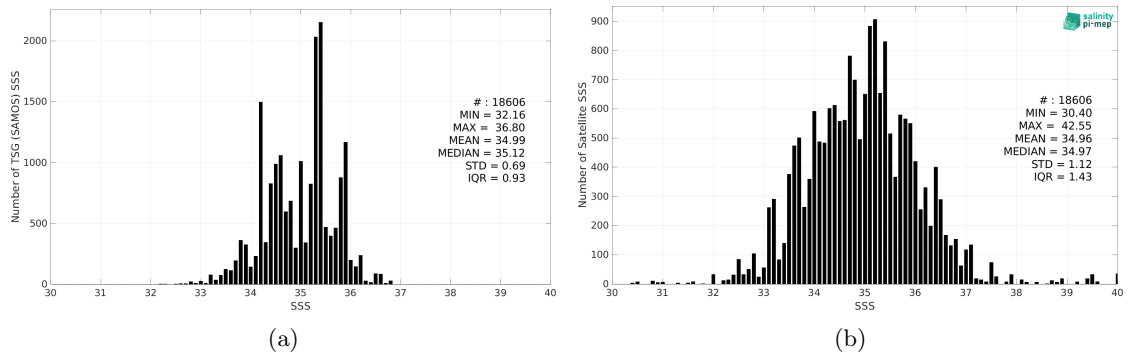
Figure 2: Histograms of SSS from TSG (SAMOS) (a) and SMAP SSS L2 v5 - 40 km (RSS) (b) considering all match-up pairs per bins of 0.1 over the Indian Ocean Pi-MEP region and for the full satellite product period.
