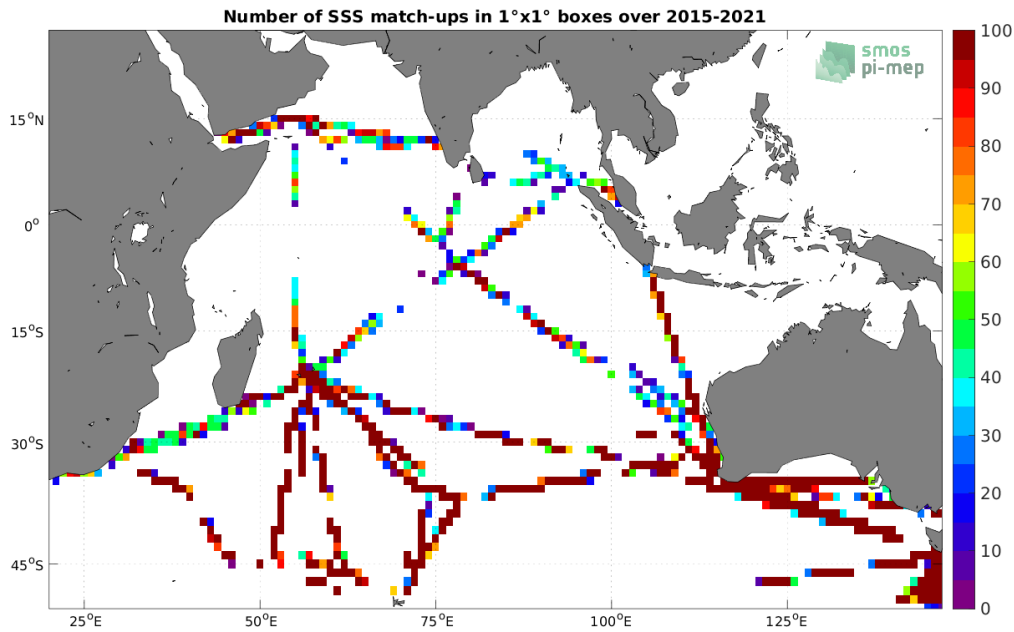
Figure 4: Number of SSS match-ups between TSG (LEGOS-DM) SSS and the SMAP SSS L2 v5 - 40 km (RSS) SSS product for the Indian Ocean Pi-MEP region over 1^\circ \times 1^\circ boxes and for the full satellite product period.
