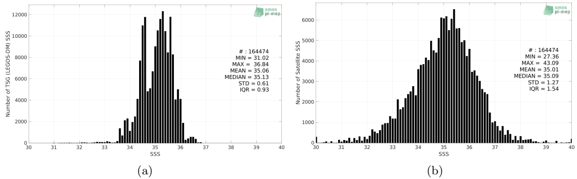
Figure 2: Histograms of SSS from TSG (LEGOS-DM) (a) and SMAP SSS L2 v5 - 40 km (RSS) (b) considering all match-up pairs per bins of 0.1 over the Indian Ocean Pi-MEP region and for the full satellite product period.
