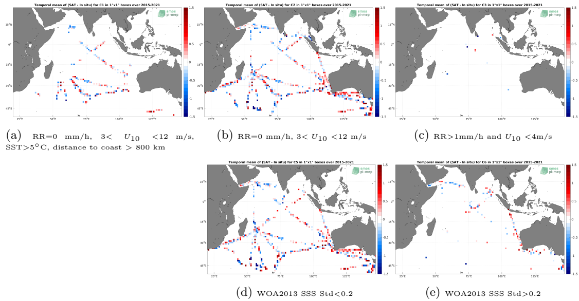
Figure 12: Temporal mean gridded over spatial boxes of size 1^\circ \times 1^\circ of \Delta SSS (SMAP SSS L2 v5 - 40 km (RSS) - TSG (LEGOS-DM)) for 5 different subdatasets corresponding to:RR=0 mm/h, 3 < U_{10} < 12 m/s, SST >5^\circ\text{C} , distance to coast > 800 km (a), RR=0 mm/h, 3 < U_{10} < 12 m/s (b), RR >1 mm/h and U_{10} < 4 m/s (c), WOA2013 SSS Std <0.2 (d), WOA2013 SSS Std >0.2 (e).
