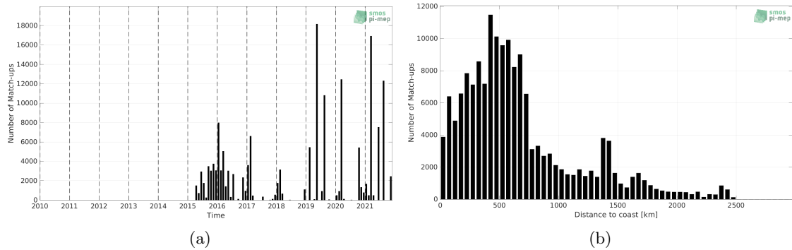
Figure 1: Number of match-ups between TSG (LEGOS-DM) and SMAP SSS L2 v5 - 40 km (RSS) SSS as a function of time (a) and as function of the distance to coast (b) over the Indian Ocean Pi-MEP region and for the full satellite product period.
