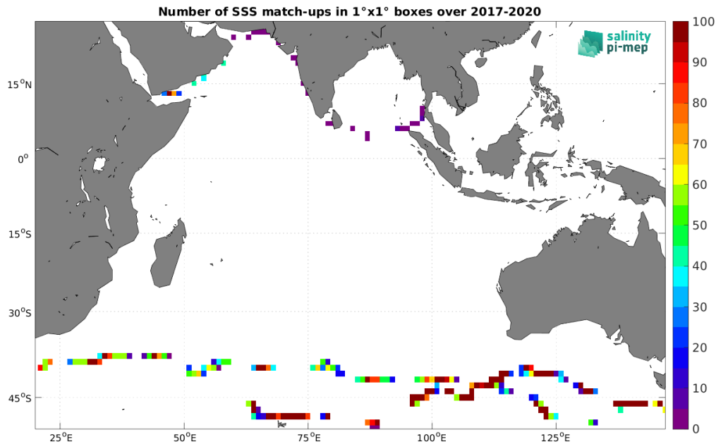
Figure 4: Number of SSS match-ups between TSG (GOSUD-Sailing-ship) SSS and the SMAP SSS L2 v5 - 40 km (RSS) SSS product for the Indian Ocean Pi-MEP region over 1^\circ \times 1^\circ boxes and for the full satellite product period.
