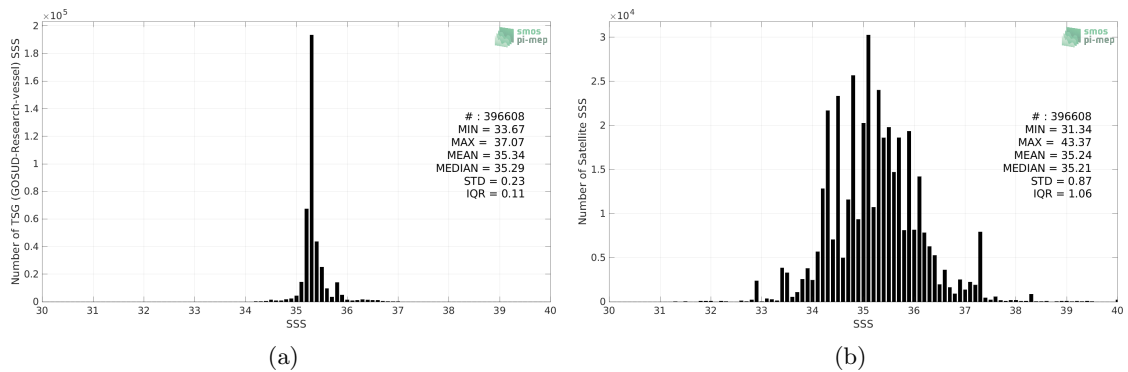
Figure 2: Histograms of SSS from TSG (GOSUD-Research-vessel) (a) and SMAP SSS L2 v5 - 40 km (RSS) (b) considering all match-up pairs per bins of 0.1 over the Indian Ocean Pi-MEP region and for the full satellite product period.
