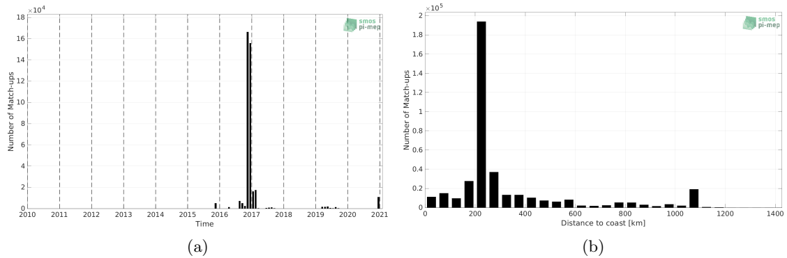
Figure 1: Number of match-ups between TSG (GOSUD-Research-vessel) and SMAP SSS L2 v5 - 40 km (RSS) SSS as a function of time (a) and as function of the distance to coast (b) over the Indian Ocean Pi-MEP region and for the full satellite product period.
