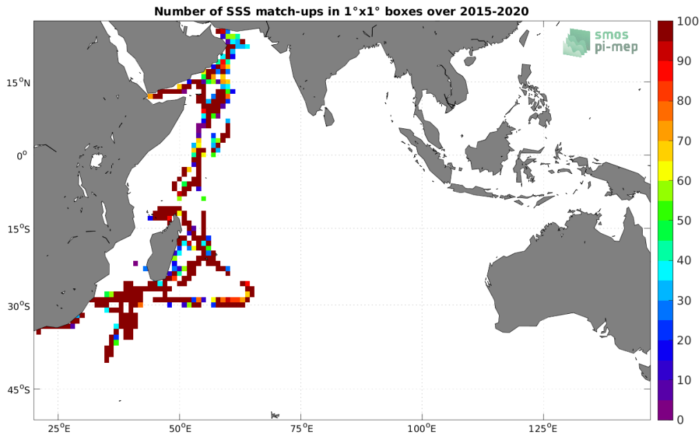
Figure 4: Number of SSS match-ups between TSG (GOSUD-Research-vessel) SSS and the SMAP SSS L2 v5 - 40 km (RSS) SSS product for the Indian Ocean Pi-MEP region over 1^\circ \times 1^\circ boxes and for the full satellite product period.
