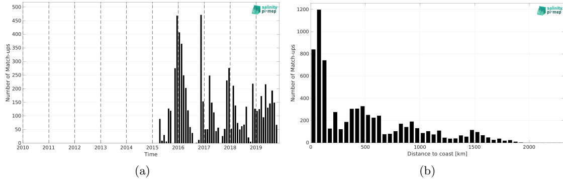
Figure 1: Number of match-ups between Marine mammals and SMAP SSS L2 v5 - 40 km (RSS) SSS as a function of time (a) and as function of the distance to coast (b) over the Indian Ocean Pi-MEP region and for the full satellite product period.
