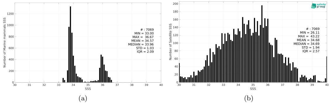
Figure 2: Histograms of SSS from Marine mammals (a) and SMAP SSS L2 v5 - 40 km (RSS) (b) considering all match-up pairs per bins of 0.1 over the Indian Ocean Pi-MEP region and for the full satellite product period.
