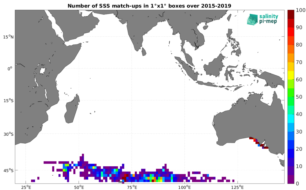
Figure 4: Number of SSS match-ups between Marine mammals SSS and the SMAP SSS L2 v5 - 40 km (RSS) SSS product for the Indian Ocean Pi-MEP region over 1^\circ \times 1^\circ boxes and for the full satellite product period.
