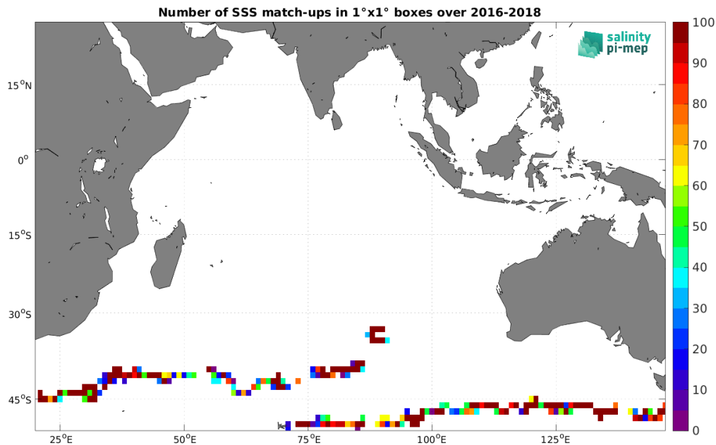
Figure 3: Number of SSS match-ups between Surface drifters SSS and the SMAP SSS L2 v5 - 40 km (RSS) SSS product for the Indian Ocean Pi-MEP region over 1^\circ \times 1^\circ boxes and for the full satellite product period.
