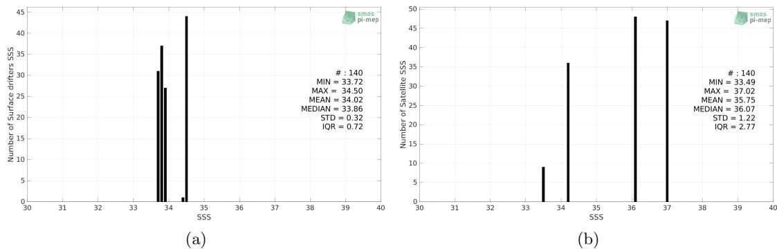
Figure 2: Histograms of SSS from Surface drifters (a) and SMAP SSS L2 v5 - 40 km (RSS) (b) considering all match-up pairs per bins of 0.1 over the Indian Ocean Pi-MEP region and for the full satellite product period.
