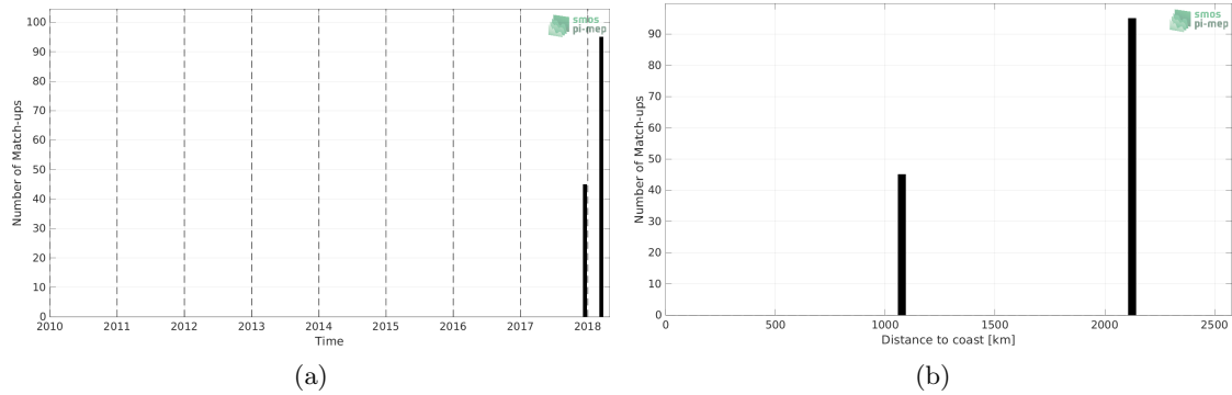
Figure 1: Number of match-ups between Surface drifters and SMAP SSS L2 v5 - 40 km (RSS) SSS as a function of time (a) and as function of the distance to coast (b) over the Indian Ocean Pi-MEP region and for the full satellite product period.
