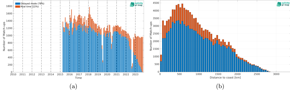
Figure 1: Number of match-ups between Argo and SMAP SSS L2 v5 - 40 km (RSS) SSS as a function of time (a) and as function of the distance to coast (b) over the Indian Ocean Pi-MEP region and for the full satellite product period.
