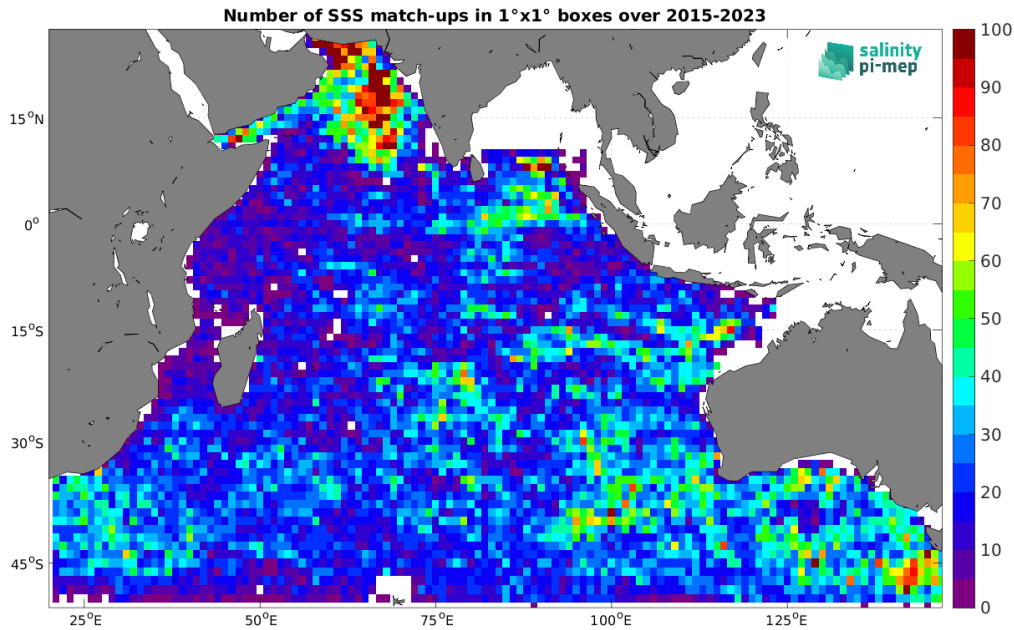
Figure 4: Number of SSS match-ups between Argo SSS and the SMAP SSS L2 v5 - 40 km (RSS) SSS product for the Indian Ocean Pi-MEP region over 1^\circ \times 1^\circ boxes and for the full satellite product period.
