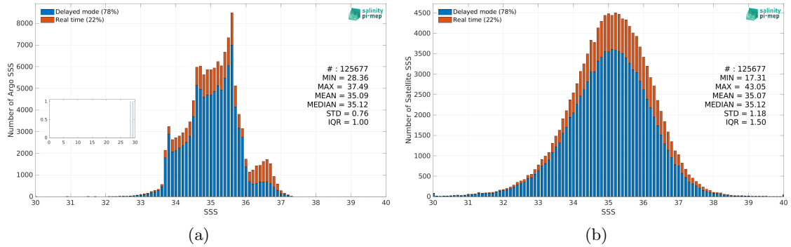
Figure 2: Histograms of SSS from Argo (a) and SMAP SSS L2 v5 - 40 km (RSS) (b) considering all match-up pairs per bins of 0.1 over the Indian Ocean Pi-MEP region and for the full satellite product period.
