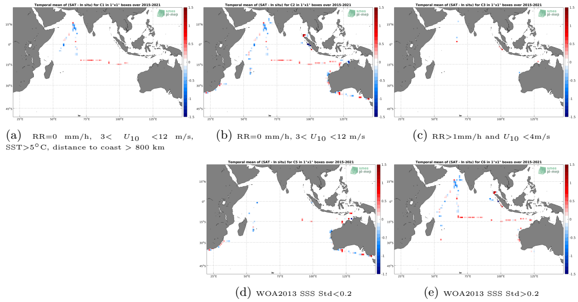
Figure 12: Temporal mean gridded over spatial boxes of size 1^\circ \times 1^\circ of \Delta SSS (SMAP SSS L2 v4 (RSS) - TSG (SAMOS)) for 5 different subdatasets corresponding to: RR=0 mm/h, 3 < U_{10} < 12 m/s, SST > 5^\circ C , distance to coast > 800 km (a), RR=0 mm/h, 3 < U_{10} < 12 m/s (b), RR > 1 mm/h and U_{10} < 4 m/s (c), WOA2013 SSS Std < 0.2 (d), WOA2013 SSS Std > 0.2 (e).
