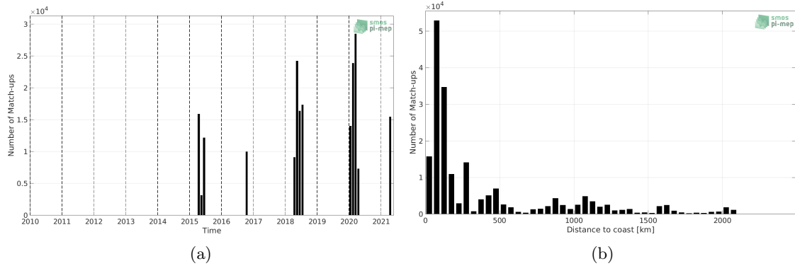
Figure 1: Number of match-ups between TSG (SAMOS) and SMAP SSS L2 v4 (RSS) SSS as a function of time (a) and as function of the distance to coast (b) over the Indian Ocean Pi-MEP region and for the full satellite product period.
