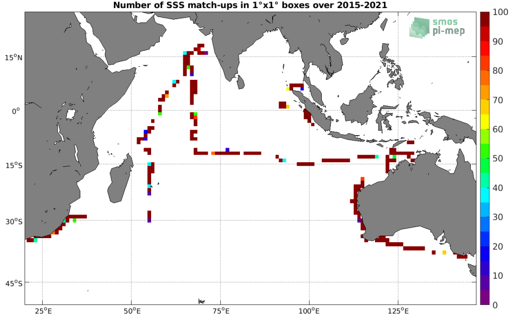
Figure 4: Number of SSS match-ups between TSG (SAMOS) SSS and the SMAP SSS L2 v4 (RSS) SSS product for the Indian Ocean Pi-MEP region over 1^\circ \times 1^\circ boxes and for the full satellite product period.
