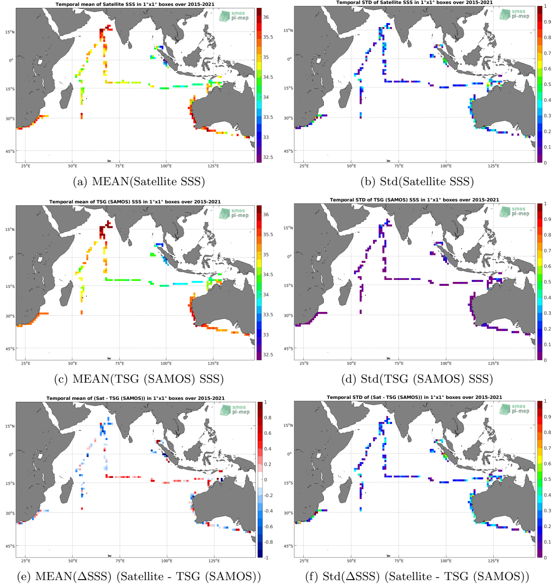
Figure 6: Temporal mean (left) and Std (right) of SSS from SMAP SSS L2 v4 (RSS) (top), TSG (SAMOS) (middle), and of \Delta SSS (Satellite - TSG (SAMOS)). Only match-up pairs are used to generate these maps.
