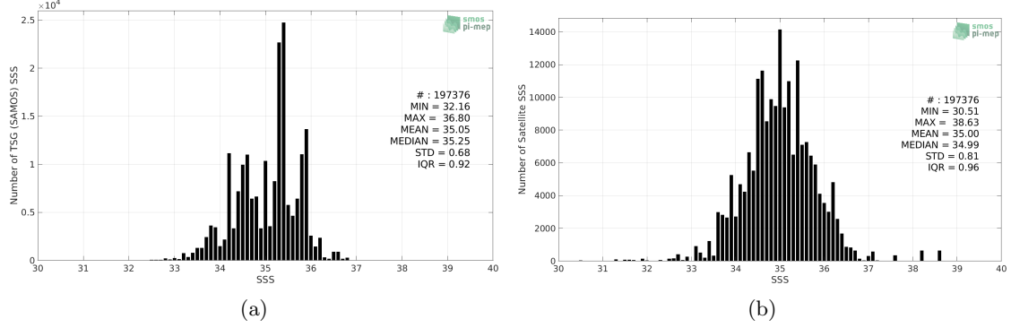
Figure 2: Histograms of SSS from TSG (SAMOS) (a) and SMAP SSS L2 v4 (RSS) (b) considering all match-up pairs per bins of 0.1 over the Indian Ocean Pi-MEP region and for the full satellite product period.
