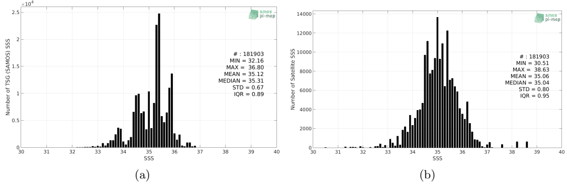
Figure 2: Histograms of SSS from TSG (SAMOS) (a) and SMAP SSS L2 v4 (RSS) (b) considering all match-up pairs per bins of 0.1 over the Indian Ocean Pi-MEP region and for the full satellite product period.
