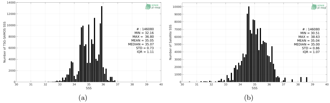
Figure 2: Histograms of SSS from TSG-SAMOS (a) and SMAP-L2-RSS-V4 (b) considering all match-up pairs per bins of 0.1 over the Indian Ocean Pi-MEP region and for the full satellite product period.
