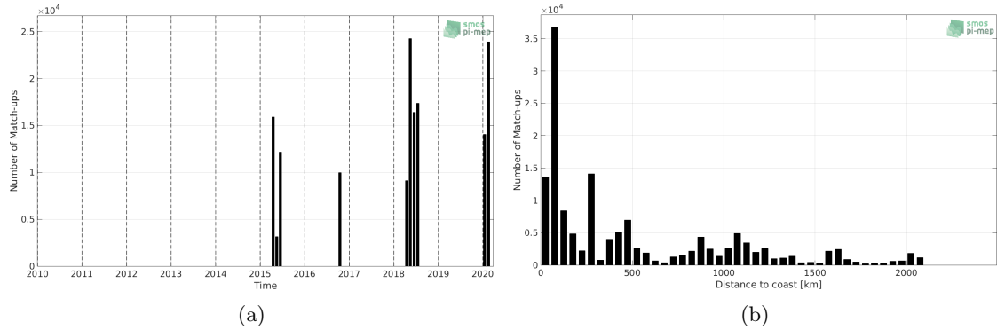
Figure 1: Number of match-ups between TSG-SAMOS and SMAP-L2-RSS-V4 SSS as a function of time (a) and as function of the distance to coast (b) over the Indian Ocean Pi-MEP region and for the full satellite product period.
