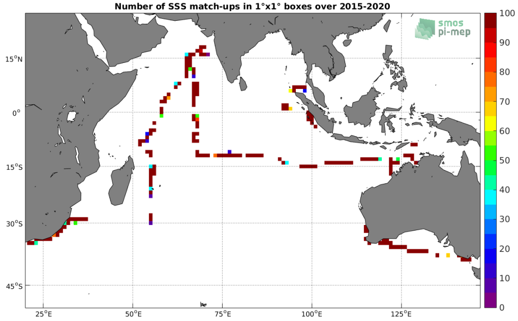
Figure 4: Number of SSS match-ups between TSG-SAMOS SSS and the SMAP-L2-RSS-V4 SSS product for the Indian Ocean Pi-MEP region over 1^\circ \times 1^\circ boxes and for the full satellite product period.
