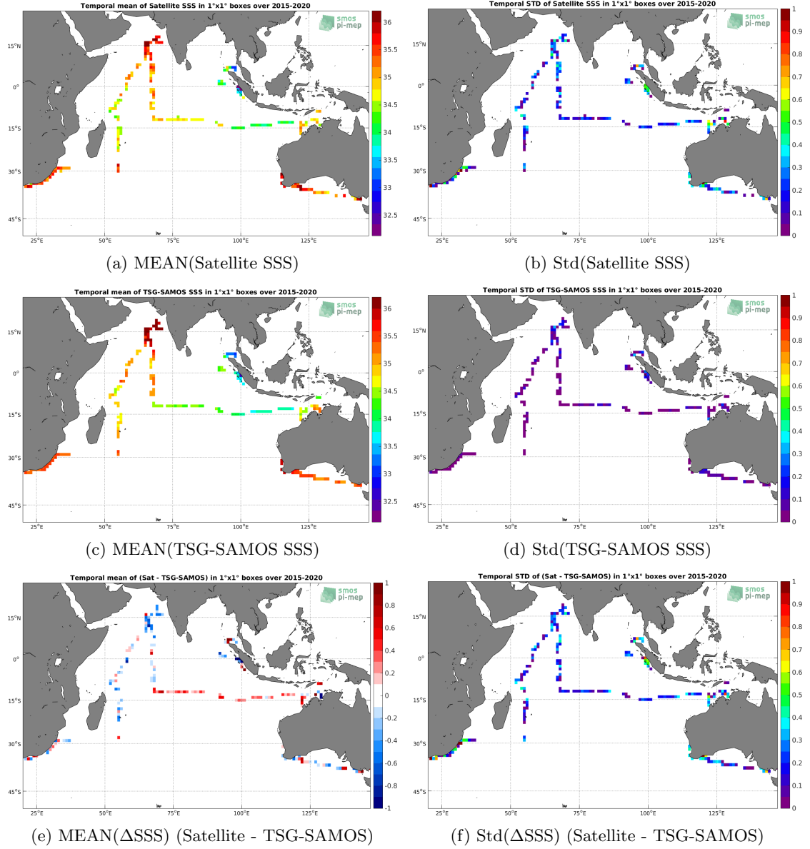
Figure 6: Temporal mean (left) and Std (right) of SSS from SMAP-L2-RSS-V4 (top), TSG-SAMOS (middle), and of \Delta SSS (Satellite - TSG-SAMOS). Only match-up pairs are used to generate these maps.
