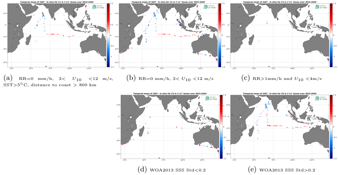
Figure 12: Temporal mean gridded over spatial boxes of size 1^\circ \times 1^\circ of \Delta SSS (SMAP-L2-RSS-V4 - TSG-SAMOS) for 5 different subdatasets corresponding to: RR=0 mm/h, 3 < U_{10} < 12 m/s, SST > 5^\circ\text{C} , distance to coast > 800 km (a), RR=0 mm/h, 3 < U_{10} < 12 m/s (b), RR > 1 mm/h and U_{10} < 4 m/s (c), WOA2013 SSS Std < 0.2 (d), WOA2013 SSS Std > 0.2 (e).
