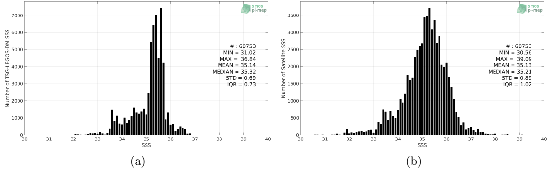
Figure 2: Histograms of SSS from TSG-LEGOS-DM (a) and SMAP-L2-RSS-V4 (b) considering all match-up pairs per bins of 0.1 over the Indian Ocean Pi-MEP region and for the full satellite product period.
