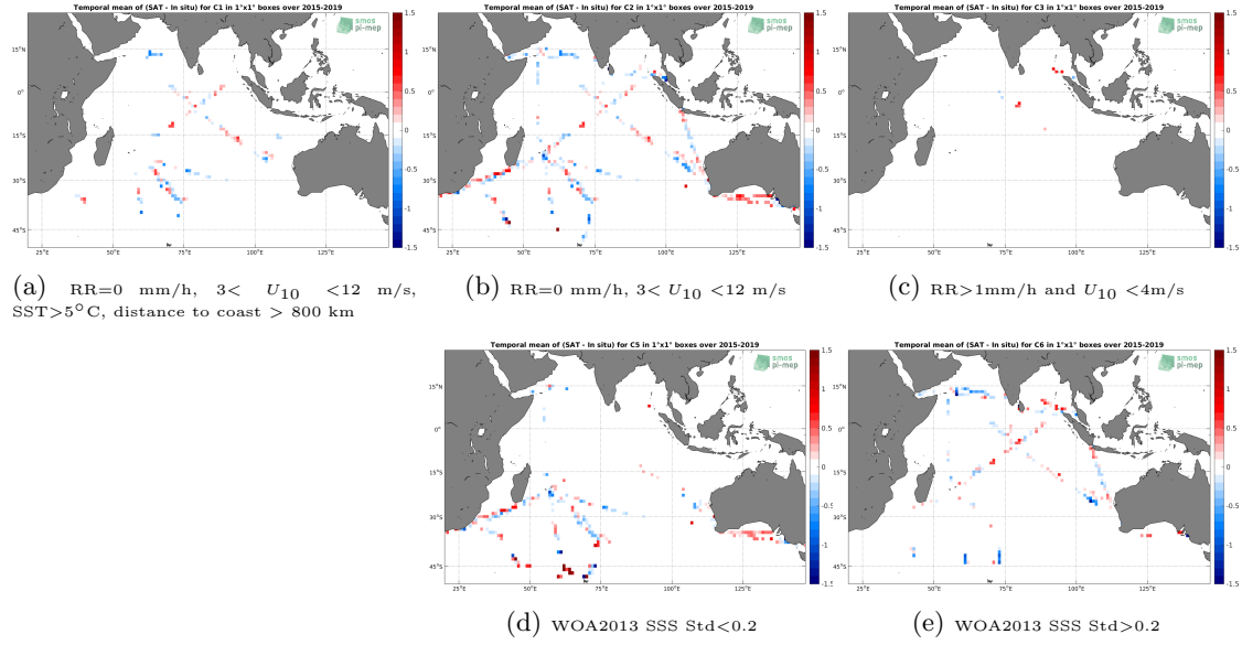
Figure 12: Temporal mean gridded over spatial boxes of size 1^\circ \times 1^\circ of \Delta SSS (SMAP-L2-RSS-V4 - TSG-LEGOS-DM) for 5 different subdatasets corresponding to: RR=0 mm/h, 3 < U_{10} < 12 m/s, SST >5^\circ C, distance to coast > 800 km (a), RR=0 mm/h, 3 < U_{10} < 12 m/s (b), RR >1 mm/h and U_{10} < 4 m/s (c), WOA2013 SSS Std <0.2 (d), WOA2013 SSS Std >0.2 (e).
