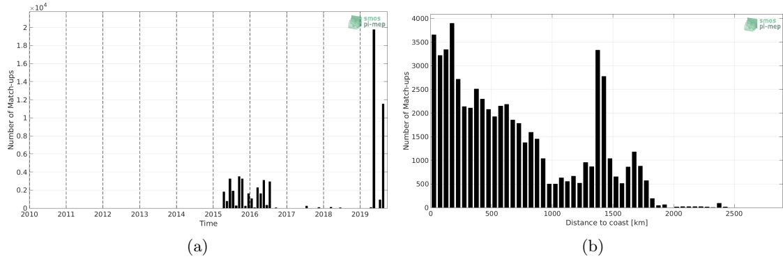
Figure 1: Number of match-ups between TSG-LEGOS-DM and SMAP-L2-RSS-V4 SSS as a function of time (a) and as function of the distance to coast (b) over the Indian Ocean Pi-MEP region and for the full satellite product period.
