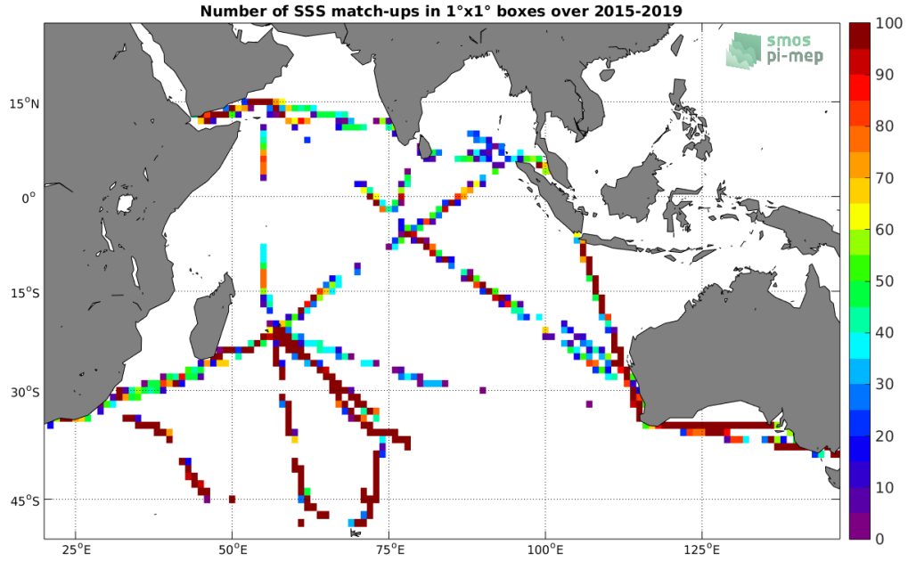
Figure 4: Number of SSS match-ups between TSG-LEGOS-DM SSS and the SMAP-L2-RSS-V4 SSS product for the Indian Ocean Pi-MEP region over 1^\circ \times 1^\circ boxes and for the full satellite product period.
