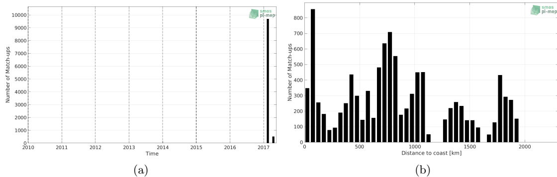
Figure 1: Number of match-ups between TSG (GOSUD-Sailing-ship) and SMAP SSS L2 v4 (RSS) SSS as a function of time (a) and as function of the distance to coast (b) over the Indian Ocean Pi-MEP region and for the full satellite product period.
