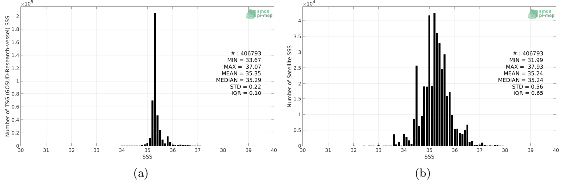
Figure 2: Histograms of SSS from TSG (GOSUD-Research-vessel) (a) and SMAP SSS L2 v4 (RSS) (b) considering all match-up pairs per bins of 0.1 over the Indian Ocean Pi-MEP region and for the full satellite product period.
