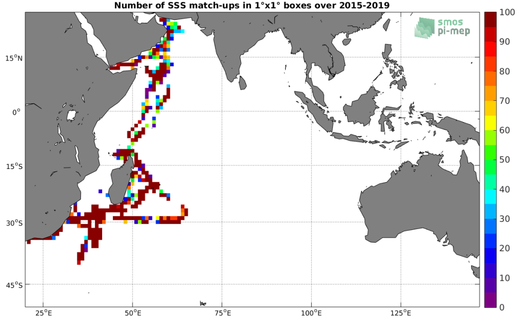
Figure 4: Number of SSS match-ups between TSG (GOSUD-Research-vessel) SSS and the SMAP SSS L2 v4 (RSS) SSS product for the Indian Ocean Pi-MEP region over 1^\circ \times 1^\circ boxes and for the full satellite product period.
