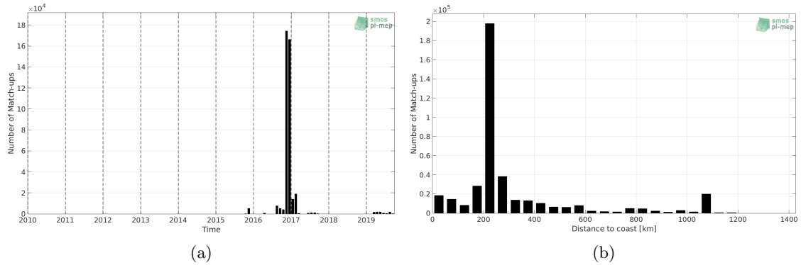
Figure 1: Number of match-ups between TSG (GOSUD-Research-vessel) and SMAP SSS L2 v4 (RSS) SSS as a function of time (a) and as function of the distance to coast (b) over the Indian Ocean Pi-MEP region and for the full satellite product period.
