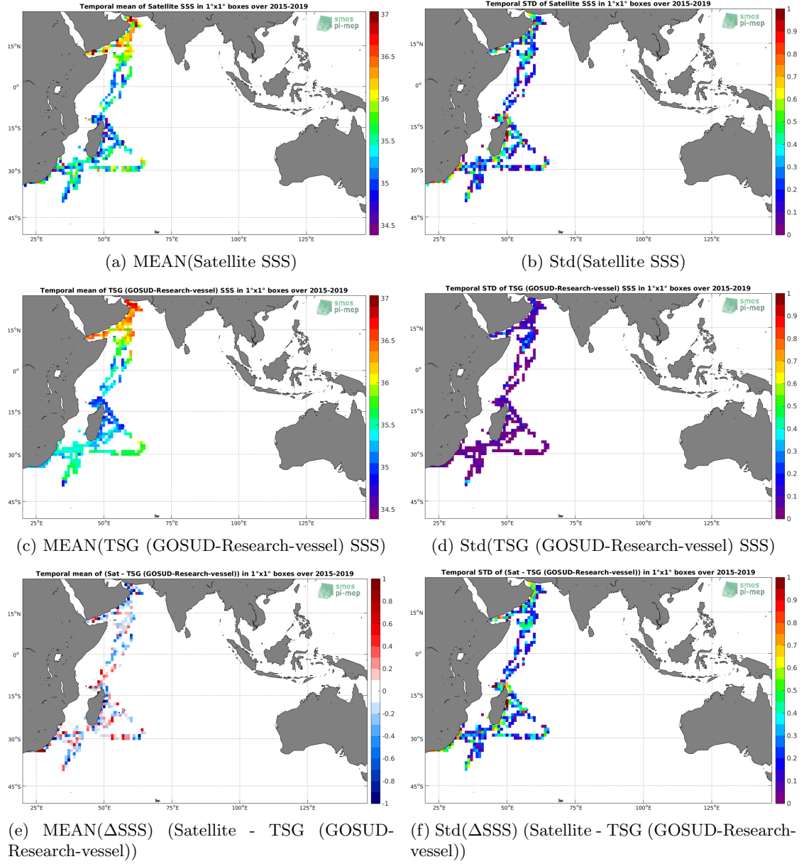
Figure 6: Temporal mean (left) and Std (right) of SSS from SMAP SSS L2 v4 (RSS) (top), TSG (GOSUD-Research-vessel) (middle), and of \Delta SSS (Satellite - TSG (GOSUD-Research-vessel)). Only match-up pairs are used to generate these maps.
