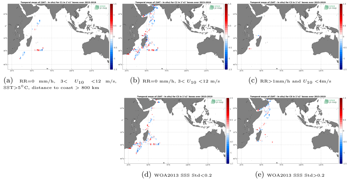
Figure 12: Temporal mean gridded over spatial boxes of size 1^\circ \times 1^\circ of \Delta SSS (SMAP SSS L2 v4 (RSS) - TSG (GOSUD-Research-vessel)) for 5 different subdatasets corresponding to: RR=0 mm/h, 3 < U_{10} < 12 m/s, SST >5^\circ C, distance to coast > 800 km (a), RR=0 mm/h, 3 < U_{10} < 12 m/s (b), RR >1 mm/h and U_{10} < 4 m/s (c), WOA2013 SSS Std <0.2 (d), WOA2013 SSS Std >0.2 (e).
