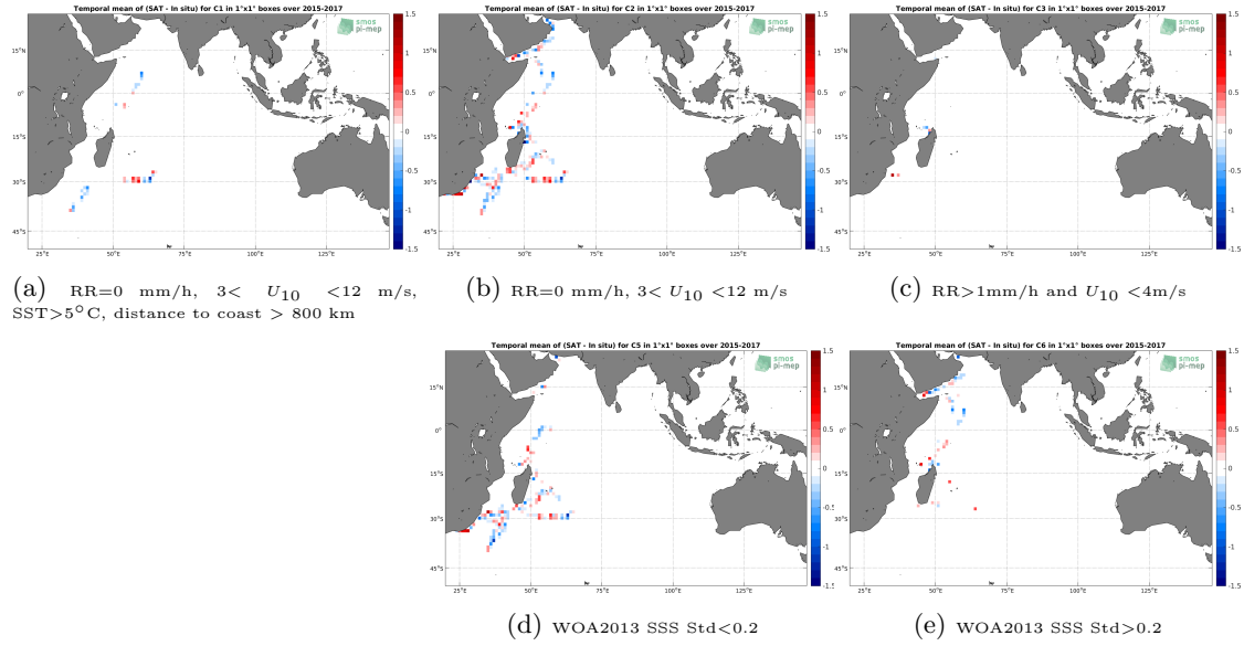
Figure 12: Temporal mean gridded over spatial boxes of size 1^\circ \times 1^\circ of \Delta SSS (SMAP-L2-RSS-V4 - TSG-GOSUD-Research-vessel) for 5 different subdatasets corresponding to: RR=0 mm/h, 3 < U_{10} < 12 m/s, SST > 5^\circ C , distance to coast > 800 km (a), RR=0 mm/h, 3 < U_{10} < 12 m/s (b), RR > 1 mm/h and U_{10} < 4 m/s (c), WOA2013 SSS Std < 0.2 (d), WOA2013 SSS Std > 0.2 (e).
