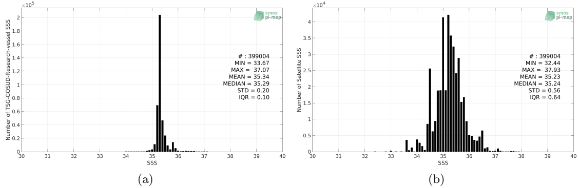
Figure 2: Histograms of SSS from TSG-GOSUD-Research-vessel (a) and SMAP-L2-RSS-V4 (b) considering all match-up pairs per bins of 0.1 over the Indian Ocean Pi-MEP region and for the full satellite product period.
