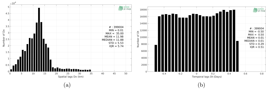
Figure 5: Histograms of the spatial (a) and temporal (b) lags between the time of the TSG-GOSUD-Research-vessel measurements and the date of the corresponding SMAP-L2-RSS-V4 SSS product.
