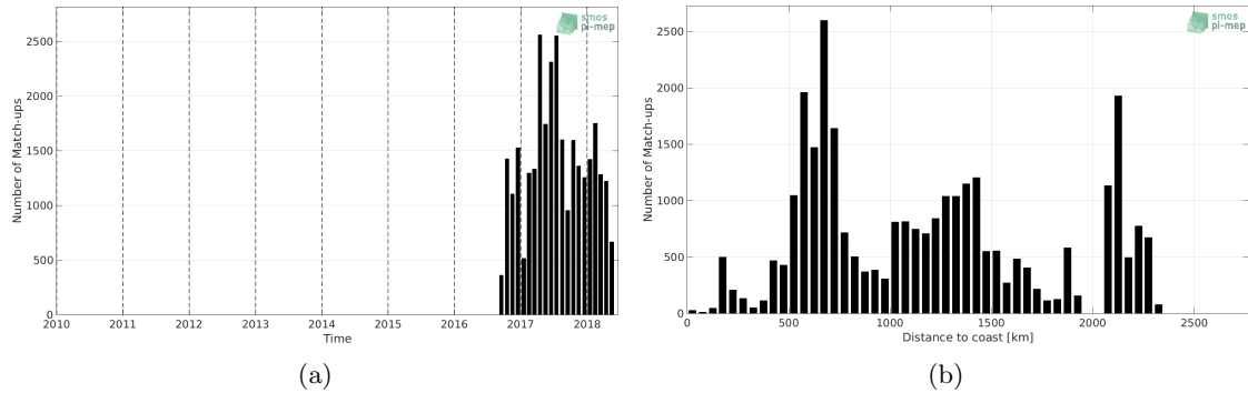
Figure 1: Number of match-ups between Surface drifters and SMAP-L2-RSS-V4 SSS as a function of time (a) and as function of the distance to coast (b) over the Indian Ocean Pi-MEP region and for the full satellite product period.
