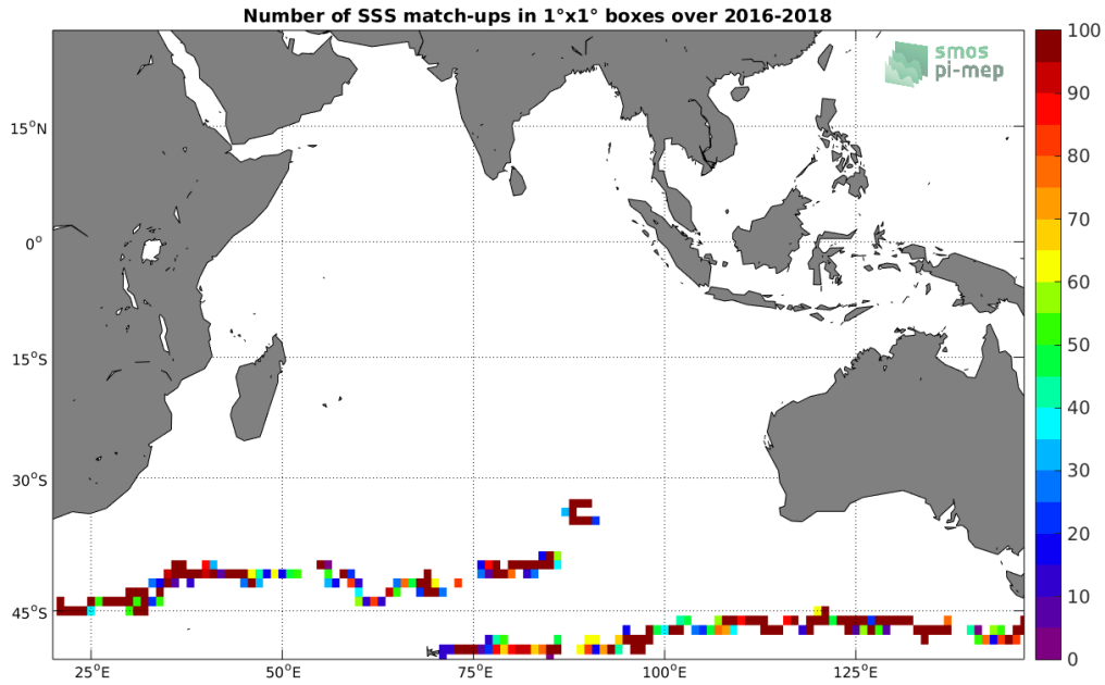
Figure 3: Number of SSS match-ups between Surface drifters SSS and the SMAP-L2-RSS-V4 SSS product for the Indian Ocean Pi-MEP region over 1°x1° boxes and for the full satellite product period.
