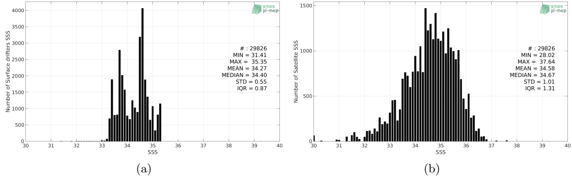
Figure 2: Histograms of SSS from Surface drifters (a) and SMAP-L2-RSS-V4 (b) considering all match-up pairs per bins of 0.1 over the Indian Ocean Pi-MEP region and for the full satellite product period.
