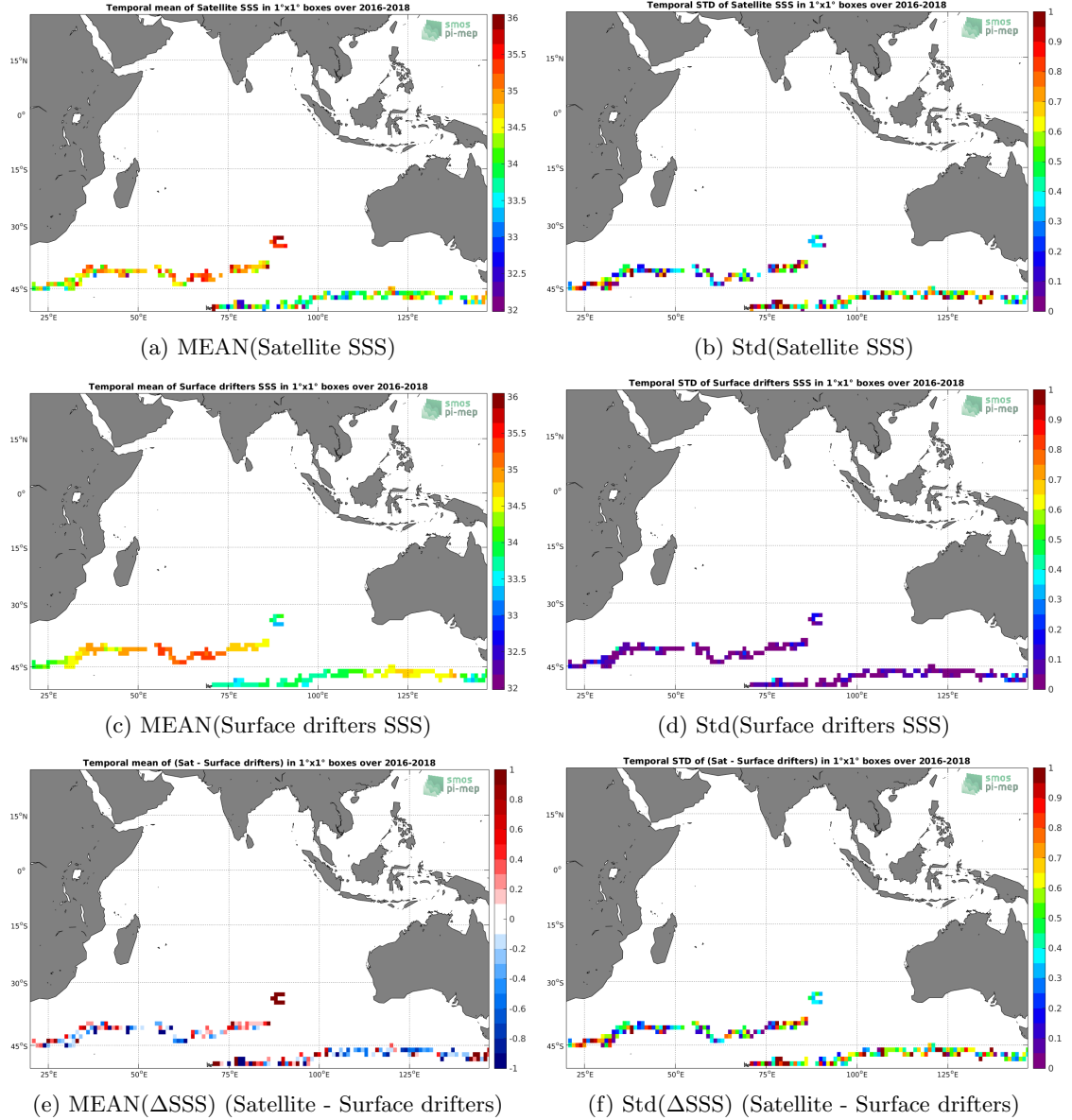
Figure 5: Temporal mean (left) and Std (right) of SSS from SMAP-L2-RSS-V4 (top), Surface drifters (middle), and of \Delta SSS (Satellite - Surface drifters). Only match-up pairs are used to generate these maps.
