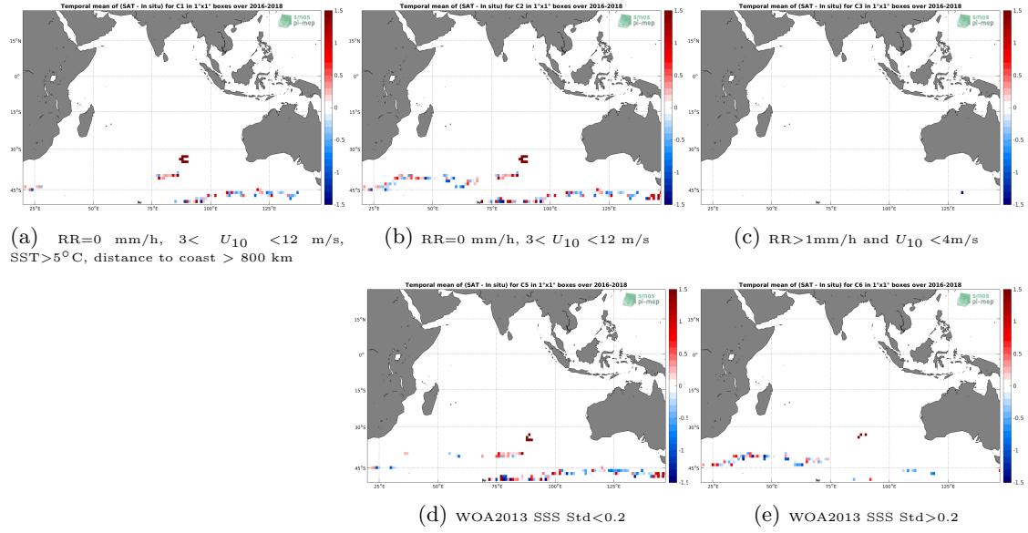
Figure 11: Temporal mean gridded over spatial boxes of size 1^\circ \times 1^\circ of \Delta SSS (SMAP-L2-RSS-V4 - Surface drifters) for 5 different subdatasets corresponding to: RR=0 mm/h, 3 < U_{10} < 12 m/s, SST > 5^\circ C , distance to coast > 800 km (a), RR=0 mm/h, 3 < U_{10} < 12 m/s (b), RR > 1 mm/h and U_{10} < 4 m/s (c), WOA2013 SSS Std < 0.2 (d), WOA2013 SSS Std > 0.2 (e).
