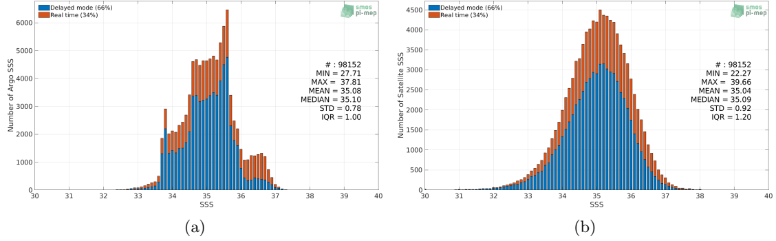
Figure 2: Histograms of SSS from Argo (a) and SMAP SSS L2 v4 (RSS) (b) considering all match-up pairs per bins of 0.1 over the Indian Ocean Pi-MEP region and for the full satellite product period.
