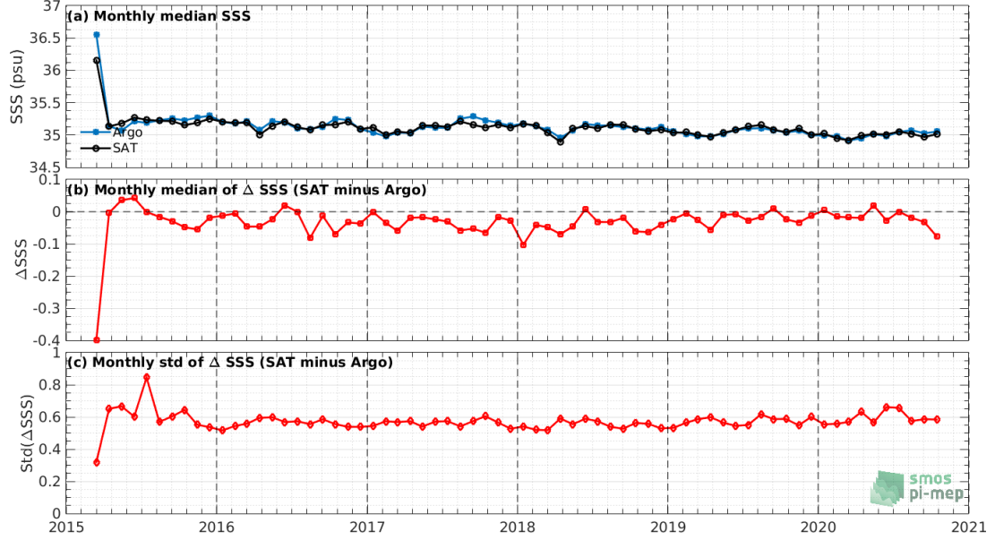
Figure 7: Time series of the monthly median SSS (top), median of \Delta\text{SSS} (Satellite - Argo) and Std of \Delta\text{SSS} (Satellite - Argo) over the Indian Ocean Pi-MEP region considering all match-ups collected by the Pi-MEP.
