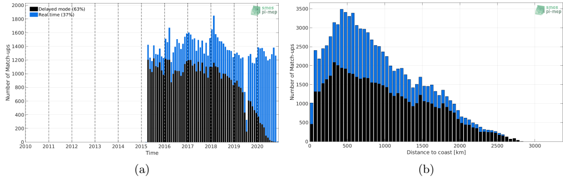
Figure 1: Number of match-ups between Argo and SMAP SSS L2 v4 (RSS) SSS as a function of time (a) and as function of the distance to coast (b) over the Indian Ocean Pi-MEP region and for the full satellite product period.
