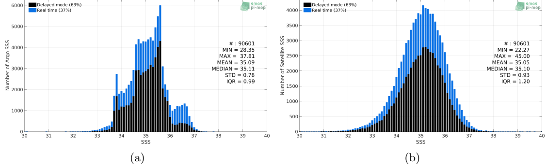
Figure 2: Histograms of SSS from Argo (a) and SMAP SSS L2 v4 (RSS) (b) considering all match-up pairs per bins of 0.1 over the Indian Ocean Pi-MEP region and for the full satellite product period.
