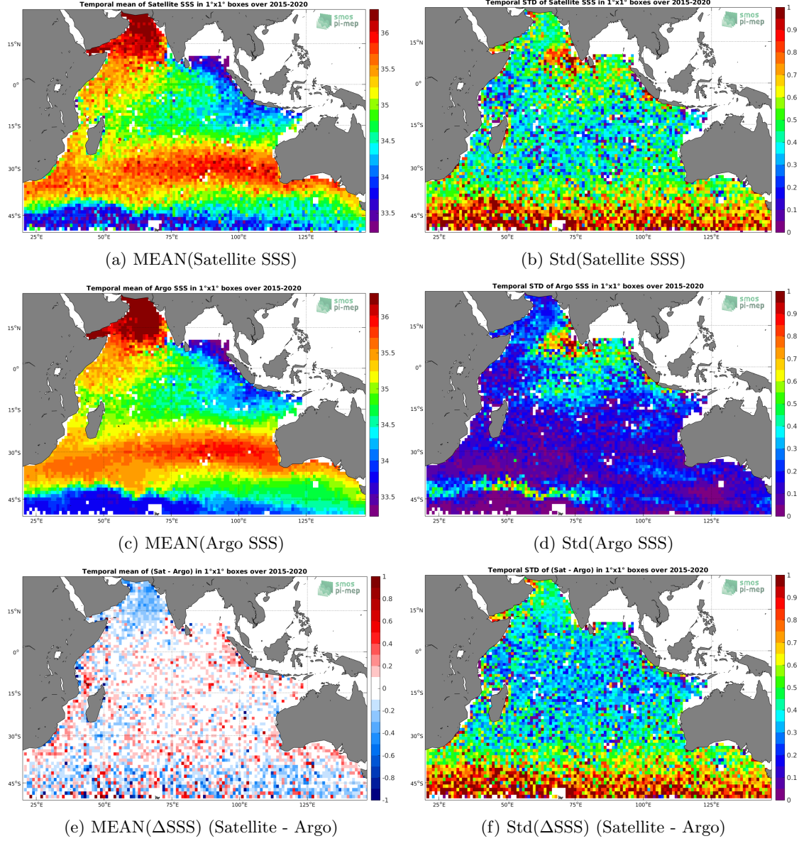
Figure 6: Temporal mean (left) and Std (right) of SSS from SMAP-L2-RSS-V4 (top), Argo (middle), and of \Delta\text{SSS} (Satellite - Argo). Only match-up pairs are used to generate these maps.
