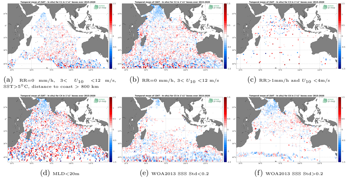
Figure 12: Temporal mean gridded over spatial boxes of size 1^\circ \times 1^\circ of \Delta SSS (SMAP-L2-RSS-V4 - Argo) for 6 different subdatasets corresponding to: RR=0 mm/h, 3 < U_{10} < 12 m/s, SST > 5^\circ C , distance to coast > 800 km (a), RR=0 mm/h, 3 < U_{10} < 12 m/s (b), RR > 1 mm/h and U_{10} < 4 m/s (c), MLD < 20 m (d), WOA2013 SSS Std < 0.2 (e), WOA2013 SSS Std > 0.2 (f).
