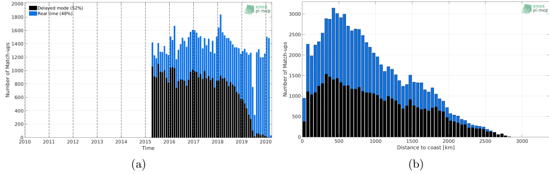
Figure 1: Number of match-ups between Argo and SMAP-L2-RSS-V4 SSS as a function of time (a) and as function of the distance to coast (b) over the Indian Ocean Pi-MEP region and for the full satellite product period.
