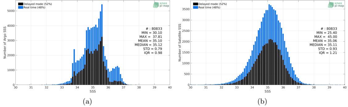
Figure 2: Histograms of SSS from Argo (a) and SMAP-L2-RSS-V4 (b) considering all match-up pairs per bins of 0.1 over the Indian Ocean Pi-MEP region and for the full satellite product period.
