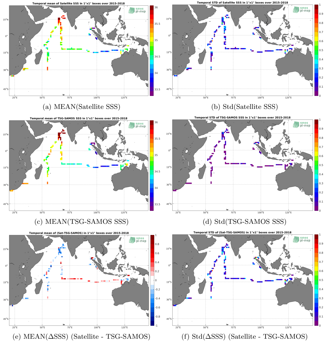
Figure 6: Temporal mean (left) and Std (right) of SSS from SMAP-L2-RSS-V3-70KM (top), TSG-SAMOS (middle), and of \Delta SSS (Satellite - TSG-SAMOS). Only match-up pairs are used to generate these maps.
