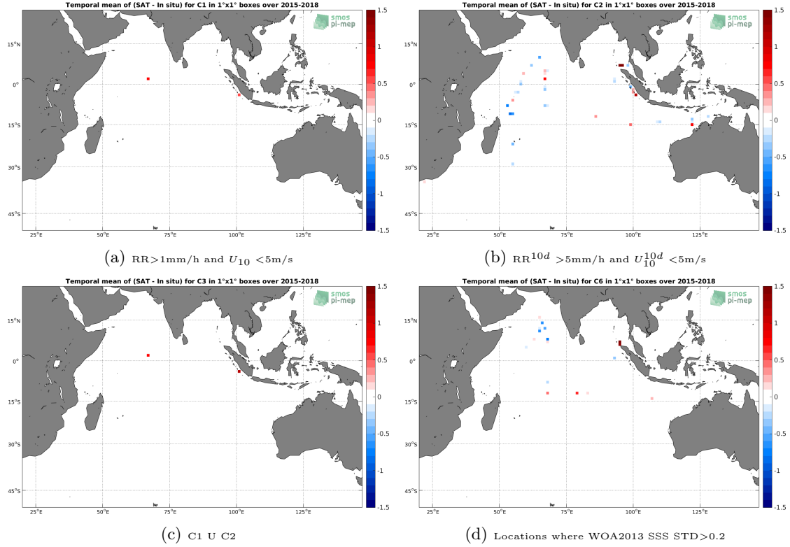
Figure 12: Temporal mean gridded over spatial boxes of size 1^\circ \times 1^\circ of \Delta SSS (SMAP-L2-RSS-V3-70KM - TSG-SAMOS) for 4 different subdatasets corresponding to: RR > 1\text{mm/h} and U_{10} < 5\text{m/s} (a), RR^{10d} > 5\text{mm/h} and U_{10}^{10d} < 5\text{m/s} (b), C1 U C2 (c), Locations where WOA2013 SSS STD > 0.2 (d).
