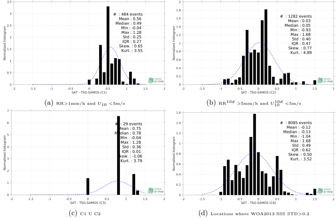
Figure 13: Normalized histogram of \Delta SSS (SMAP-L2-RSS-V3-70KM - TSG-SAMOS) for 6 different subdatasets corresponding to: RR > 1\text{mm/h} and U_{10} < 5\text{m/s} (a), RR^{10d} > 5\text{mm/h} and U_{10}^{10d} < 5\text{m/s} (b), C1 U C2 (c), Locations where WOA2013 SSS STD > 0.2 (d).
