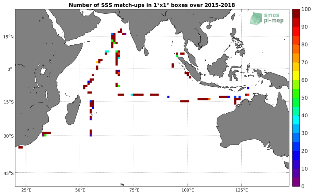
Figure 4: Number of SSS match-ups between TSG-SAMOS SSS and the SMAP-L2-RSS-V3-70KM SSS product for the Indian Ocean Pi-MEP region over 1^\circ \times 1^\circ boxes and for the full satellite product period.
