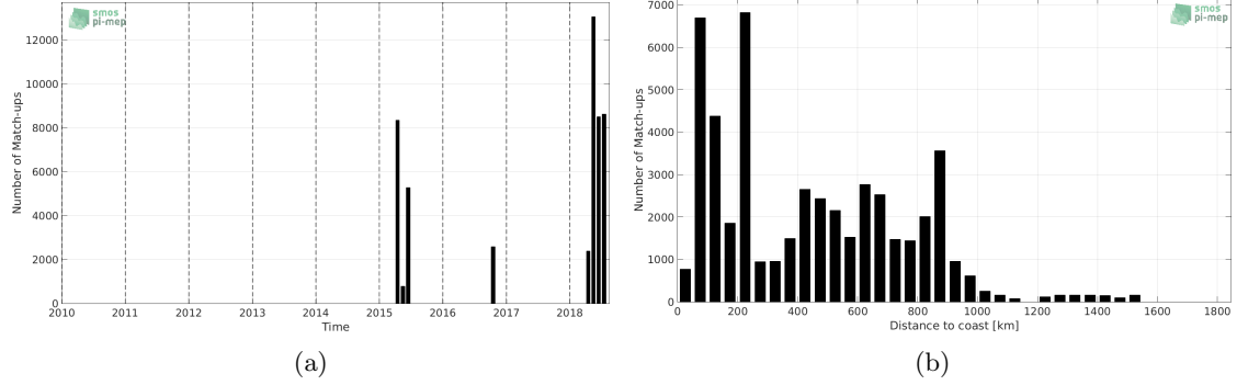
Figure 1: Number of match-ups between TSG-SAMOS and SMAP-L2-RSS-V3-70KM SSS as a function of time (a) and as function of the distance to coast (b) over the Indian Ocean Pi-MEP region and for the full satellite product period.
