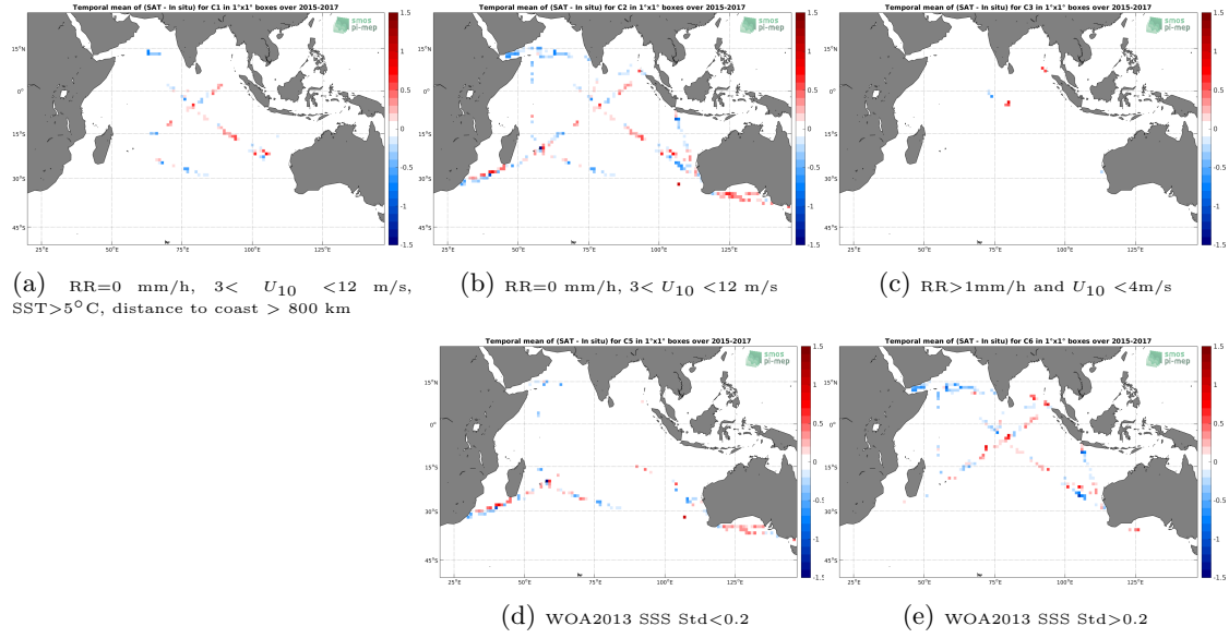
Figure 12: Temporal mean gridded over spatial boxes of size 1^\circ \times 1^\circ of \Delta SSS (SMAP-L2-RSS-V3-70KM - TSG-LEGOS-DM) for 5 different subdatasets corresponding to: RR=0 mm/h, 3 < U_{10} < 12 m/s, SST >5^\circ\text{C} , distance to coast > 800 km (a), RR=0 mm/h, 3 < U_{10} < 12 m/s (b), RR >1 mm/h and U_{10} < 4 m/s (c), WOA2013 SSS Std <0.2 (d), WOA2013 SSS Std >0.2 (e).
