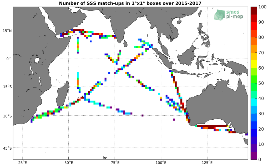
Figure 4: Number of SSS match-ups between TSG-LEGOS-DM SSS and the SMAP-L2-RSS-V3-70KM SSS product for the Indian Ocean Pi-MEP region over 1°x1° boxes and for the full satellite product period.
