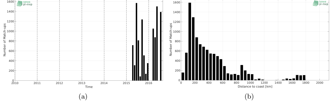
Figure 1: Number of match-ups between TSG-LEGOS-DM and SMAP-L2-RSS-V3-70KM SSS as a function of time (a) and as function of the distance to coast (b) over the Indian Ocean Pi-MEP region and for the full satellite product period.
