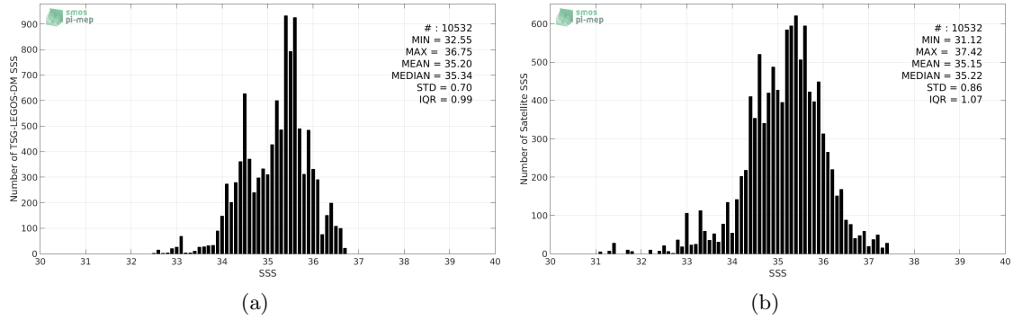
Figure 2: Histograms of SSS from TSG-LEGOS-DM (a) and SMAP-L2-RSS-V3-70KM (b) considering all match-up pairs per bins of 0.1 over the Indian Ocean Pi-MEP region and for the full satellite product period.
