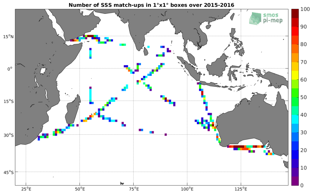
Figure 4: Number of SSS match-ups between TSG-LEGOS-DM SSS and the SMAP-L2-RSS-V3-70KM SSS product for the Indian Ocean Pi-MEP region over 1^\circ \times 1^\circ boxes and for the full satellite product period.
