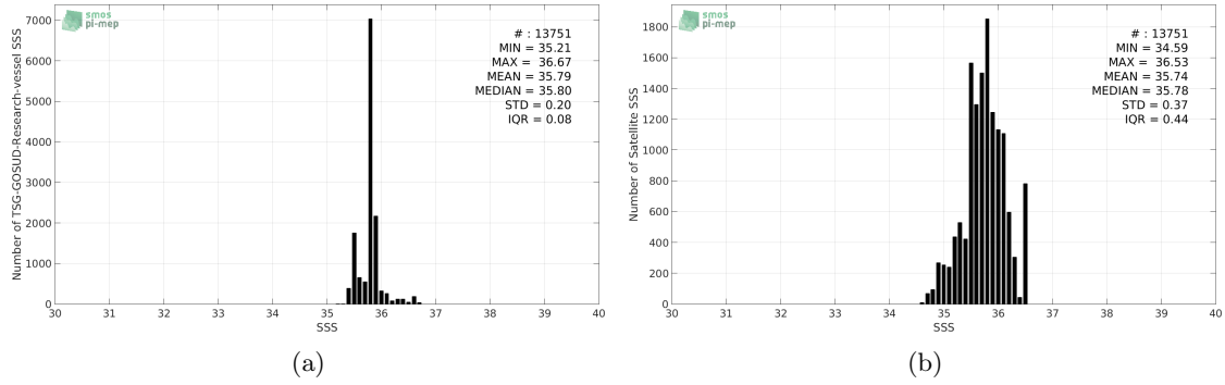
Figure 2: Histograms of SSS from TSG-GOSUD-Research-vessel (a) and SMAP-L2-RSS-V3-70KM (b) considering all match-up pairs per bins of 0.1 over the Indian Ocean Pi-MEP region and for the full satellite product period.
