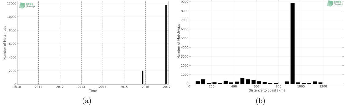
Figure 1: Number of match-ups between TSG-GOSUD-Research-vessel and SMAP-L2-RSS-V3-70KM SSS as a function of time (a) and as function of the distance to coast (b) over the Indian Ocean Pi-MEP region and for the full satellite product period.
