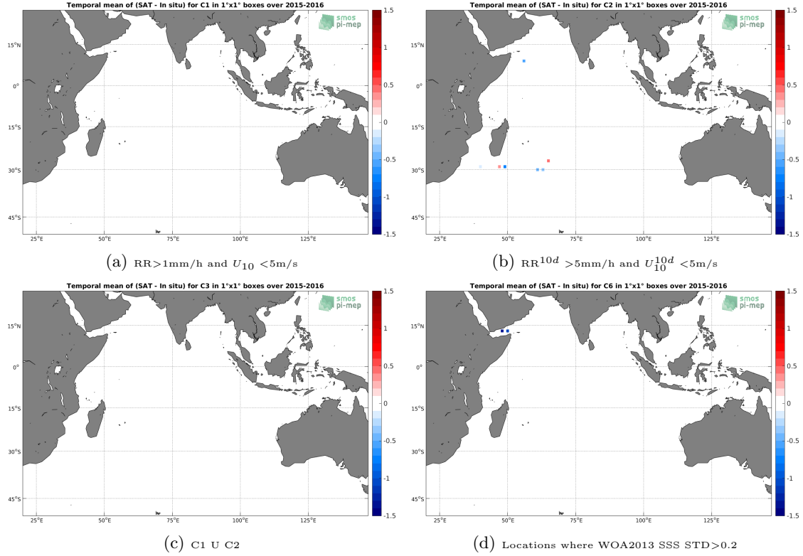
Figure 12: Temporal mean gridded over spatial boxes of size 1^\circ \times 1^\circ of \Delta SSS (SMAP-L2-RSS-V3-70KM - TSG-GOSUD-Research-vessel) for 4 different subdatasets corresponding to: RR > 1\text{mm/h} and U_{10} < 5\text{m/s} (a), RR^{10d} > 5\text{mm/h} and U_{10}^{10d} < 5\text{m/s} (b), C1 U C2 (c), Locations where WOA2013 SSS STD > 0.2 (d).
