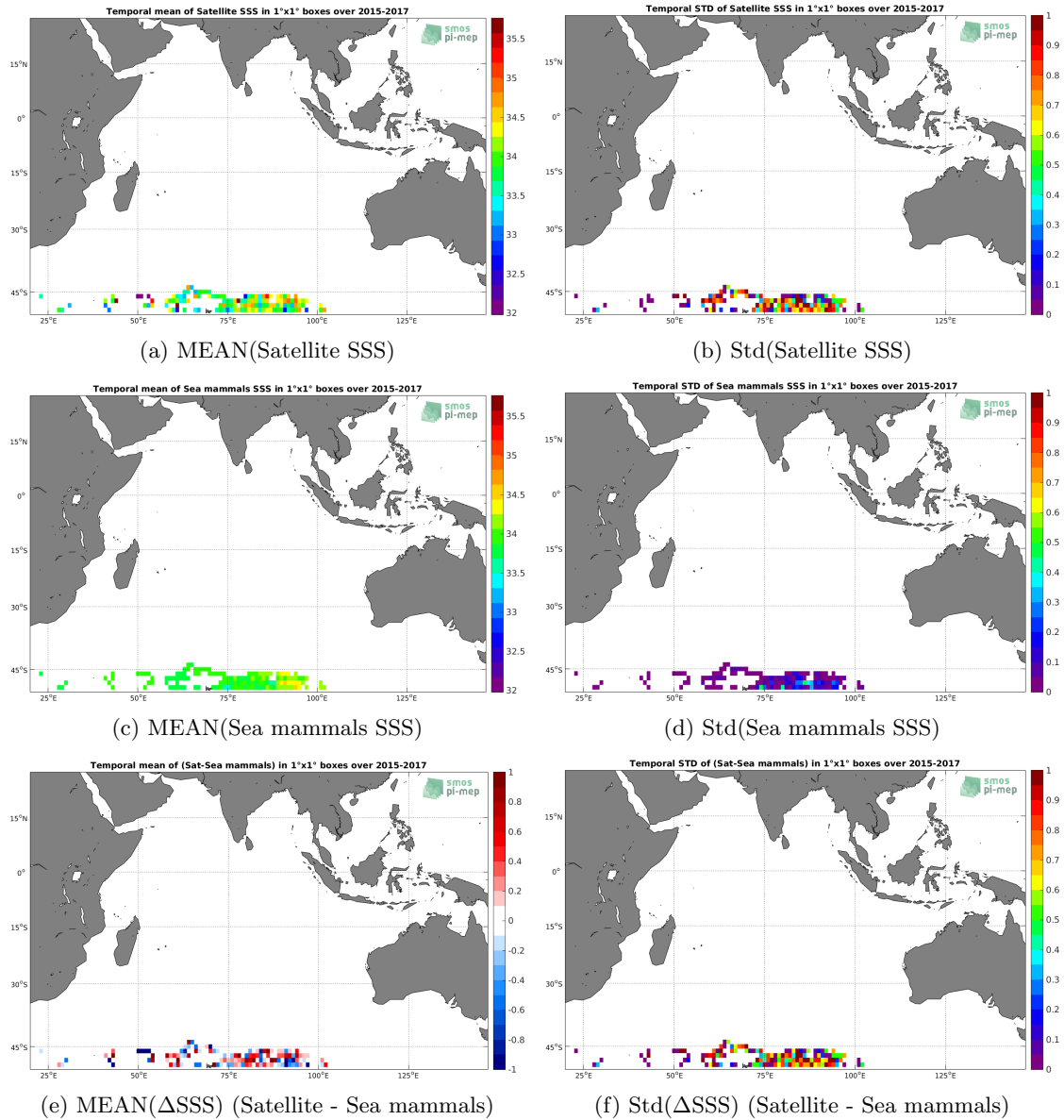
Figure 6: Temporal mean (left) and Std (right) of SSS from SMAP-L2-RSS-V3-70KM (top), Sea mammals (middle), and of \Delta SSS (Satellite - Sea mammals). Only match-up pairs are used to generate these maps.
