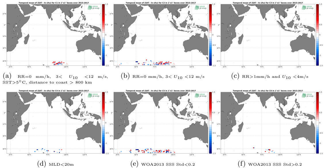
Figure 12: Temporal mean gridded over spatial boxes of size 1^\circ \times 1^\circ of \Delta SSS (SMAP-L2-RSS-V3-70KM - Sea mammals) for 6 different subdatasets corresponding to:RR=0 mm/h, 3 < U_{10} < 12 m/s, SST > 5^\circ C, distance to coast > 800 km (a), RR=0 mm/h, 3 < U_{10} < 12 m/s (b), RR > 1 mm/h and U_{10} < 4 m/s (c),MLD < 20 m (d),WOA2013 SSS Std < 0.2 (e),WOA2013 SSS Std > 0.2 (f).
