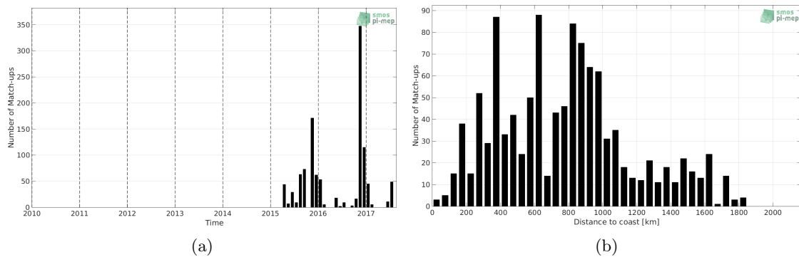
Figure 1: Number of match-ups between Sea mammals and SMAP-L2-RSS-V3-70KM SSS as a function of time (a) and as function of the distance to coast (b) over the Indian Ocean Pi-MEP region and for the full satellite product period.
