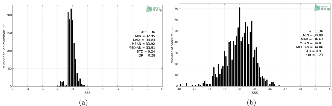
Figure 2: Histograms of SSS from Sea mammals (a) and SMAP-L2-RSS-V3-70KM (b) considering all match-up pairs per bins of 0.1 over the Indian Ocean Pi-MEP region and for the full satellite product period.
