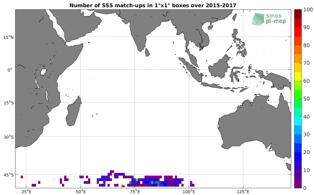
Figure 4: Number of SSS match-ups between Sea mammals SSS and the SMAP-L2-RSS-V3-70KM SSS product for the Indian Ocean Pi-MEP region over 1°x1° boxes and for the full satellite product period.
