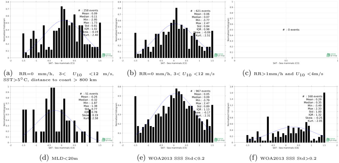
Figure 13: Normalized histogram of \Delta SSS (SMAP-L2-RSS-V3-70KM - Sea mammals) for 6 different subdatasets corresponding to: RR=0 mm/h, 3 < U_{10} < 12 m/s, SST>5°C, distance to coast > 800 km (a), RR=0 mm/h, 3 < U_{10} < 12 m/s (b), RR>1mm/h and U_{10} < 4 m/s (c), MLD<20m (d), WOA2013 SSS Std<0.2 (e), WOA2013 SSS Std>0.2 (f).
