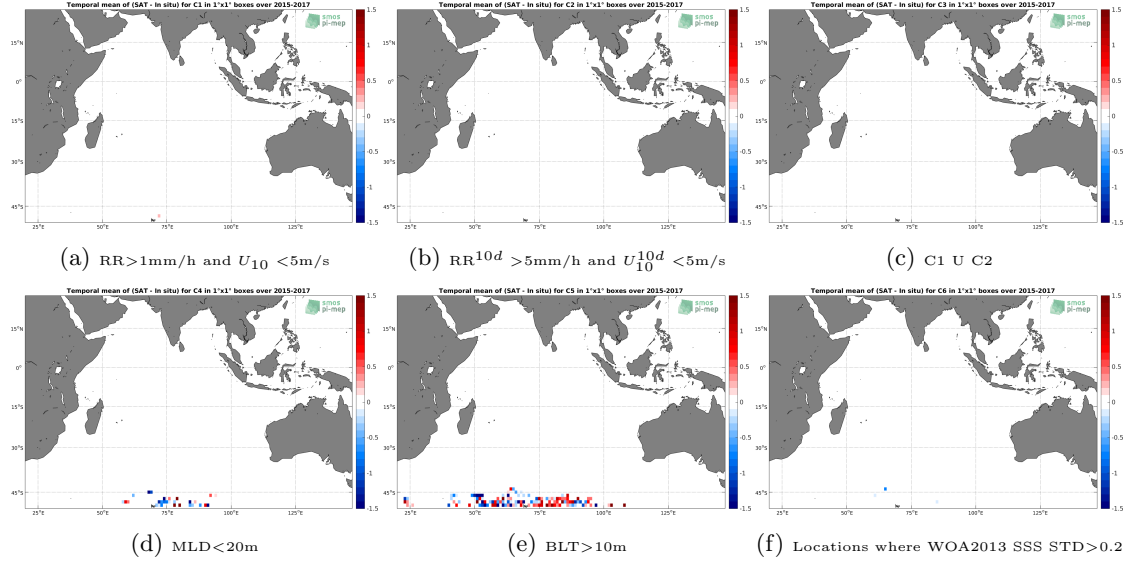
Figure 12: Temporal mean gridded over spatial boxes of size 1^\circ \times 1^\circ of \Delta\text{SSS} (SMAP-L2-RSS-V3-70KM - Sea mammals) for 6 different subdatasets corresponding to: RR > 1\text{mm/h} and U_{10} < 5\text{m/s} (a), RR^{10d} > 5\text{mm/h} and U_{10}^{10d} < 5\text{m/s} (b), C1 U C2 (c), MLD < 20\text{m} (d), BLT > 10\text{m} (e), Locations where WOA2013 SSS STD > 0.2 (f).
