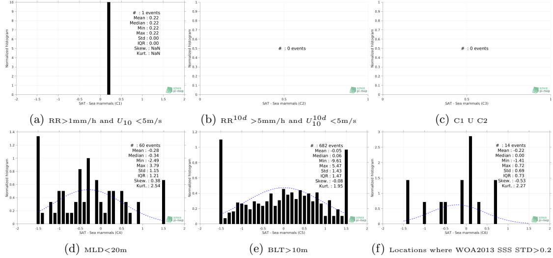
Figure 13: Normalized histogram of \Delta SSS (SMAP-L2-RSS-V3-70KM - Sea mammals) for 6 different subdatasets corresponding to: RR > 1\text{mm/h} and U_{10} < 5\text{m/s} (a), RR^{10d} > 5\text{mm/h} and U_{10}^{10d} < 5\text{m/s} (b), C1 \cup C2 (c), MLD < 20\text{m} (d), BLT > 10\text{m} (e), Locations where WOA2013 SSS STD > 0.2 (f).
