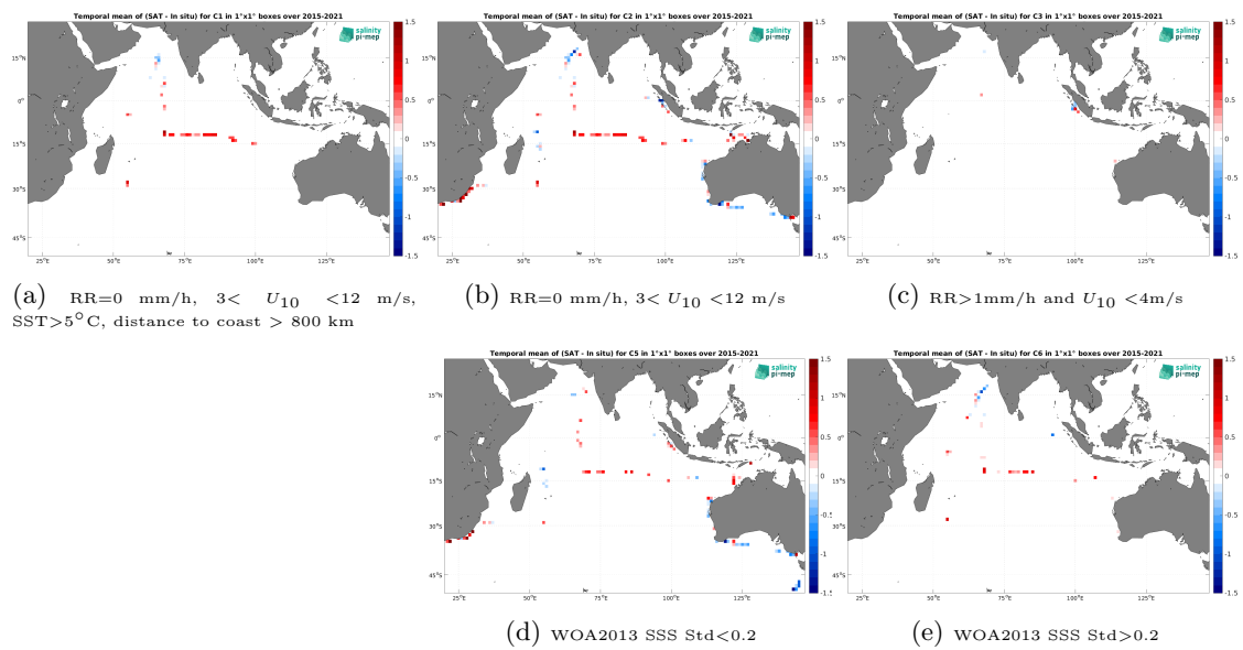
Figure 14: Temporal mean gridded over spatial boxes of size 1^\circ \times 1^\circ of \Delta SSS (SMAP SSS L2 v5.0 (JPL) - TSG (SAMOS)) for 5 different subdatasets corresponding to:RR=0 mm/h, 3 < U_{10} < 12 m/s, SST >5^\circ C, distance to coast > 800 km (a), RR=0 mm/h, 3 < U_{10} < 12 m/s (b), RR >1 mm/h and U_{10} < 4 m/s (c), WOA2013 SSS Std <0.2 (d), WOA2013 SSS Std >0.2 (e).
