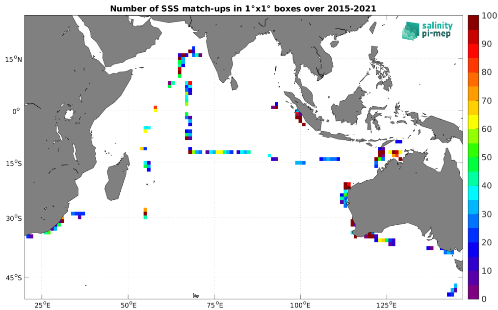
Figure 5: Number of SSS match-ups between TSG (SAMOS) SSS and the SMAP SSS L2 v5.0 (JPL) SSS product for the Indian Ocean Pi-MEP region over 1^\circ \times 1^\circ boxes and for the full satellite product period.
