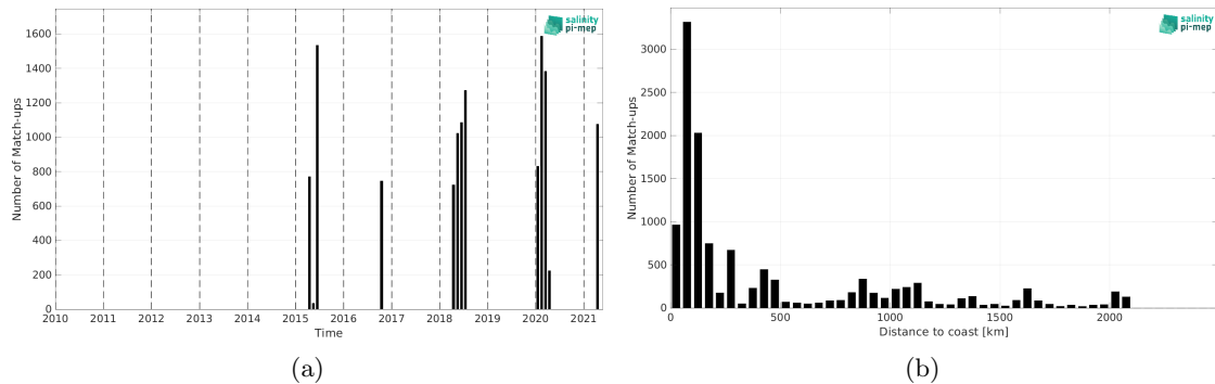
Figure 2: Number of match-ups between TSG (SAMOS) and SMAP SSS L2 v5.0 (JPL) SSS as a function of time (a) and as function of the distance to coast (b) over the Indian Ocean Pi-MEP region and for the full satellite product period.
