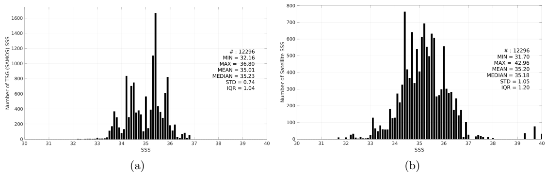
Figure 3: Histograms of SSS from TSG (SAMOS) (a) and SMAP SSS L2 v5.0 (JPL) (b) considering all match-up pairs per bins of 0.1 over the Indian Ocean Pi-MEP region and for the full satellite product period.
