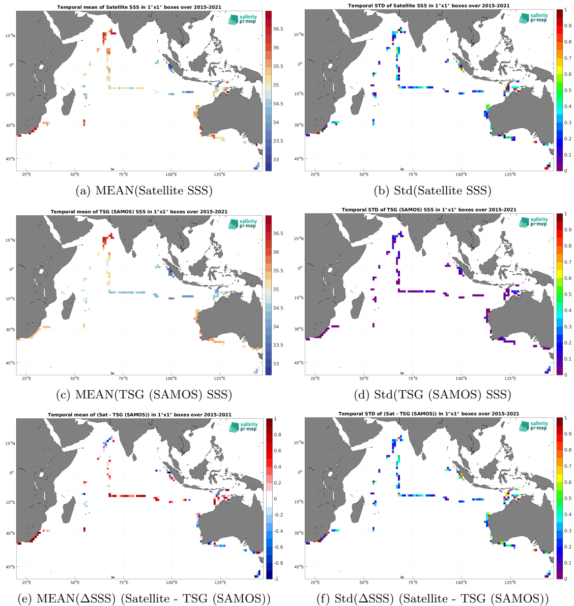
Figure 7: Temporal mean (left) and Std (right) of SSS from SMAP SSS L2 v5.0 (JPL) (top), TSG (SAMOS) (middle), and of \Delta SSS (Satellite - TSG (SAMOS)). Only match-up pairs are used to generate these maps.
