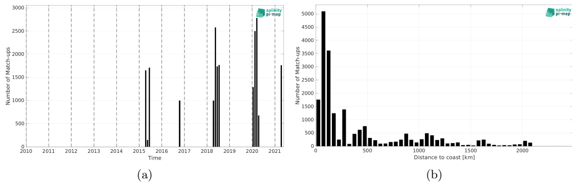
Figure 1: Number of match-ups between TSG (SAMOS) and SMAP SSS L2 v5.0 (JPL) SSS as a function of time (a) and as function of the distance to coast (b) over the Indian Ocean Pi-MEP region and for the full satellite product period.
