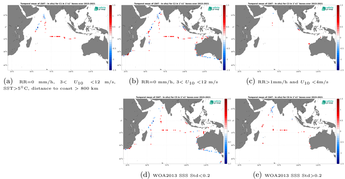
Figure 12: Temporal mean gridded over spatial boxes of size 1^\circ \times 1^\circ of \Delta SSS (SMAP SSS L2 v5.0 (JPL) - TSG (SAMOS)) for 5 different subdatasets corresponding to:RR=0 mm/h, 3 < U_{10} < 12 m/s, SST >5^\circ C, distance to coast > 800 km (a), RR=0 mm/h, 3 < U_{10} < 12 m/s (b), RR >1 mm/h and U_{10} < 4 m/s (c), WOA2013 SSS Std <0.2 (d), WOA2013 SSS Std >0.2 (e).
