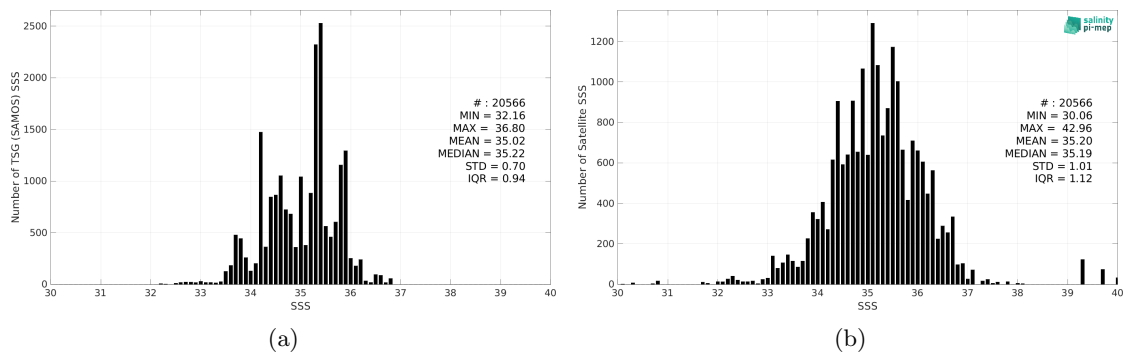
Figure 2: Histograms of SSS from TSG (SAMOS) (a) and SMAP SSS L2 v5.0 (JPL) (b) considering all match-up pairs per bins of 0.1 over the Indian Ocean Pi-MEP region and for the full satellite product period.
