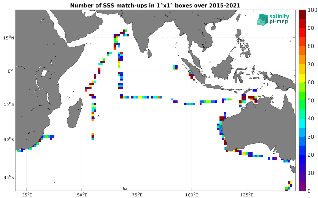
Figure 4: Number of SSS match-ups between TSG (SAMOS) SSS and the SMAP SSS L2 v5.0 (JPL) SSS product for the Indian Ocean Pi-MEP region over 1^\circ \times 1^\circ boxes and for the full satellite product period.
