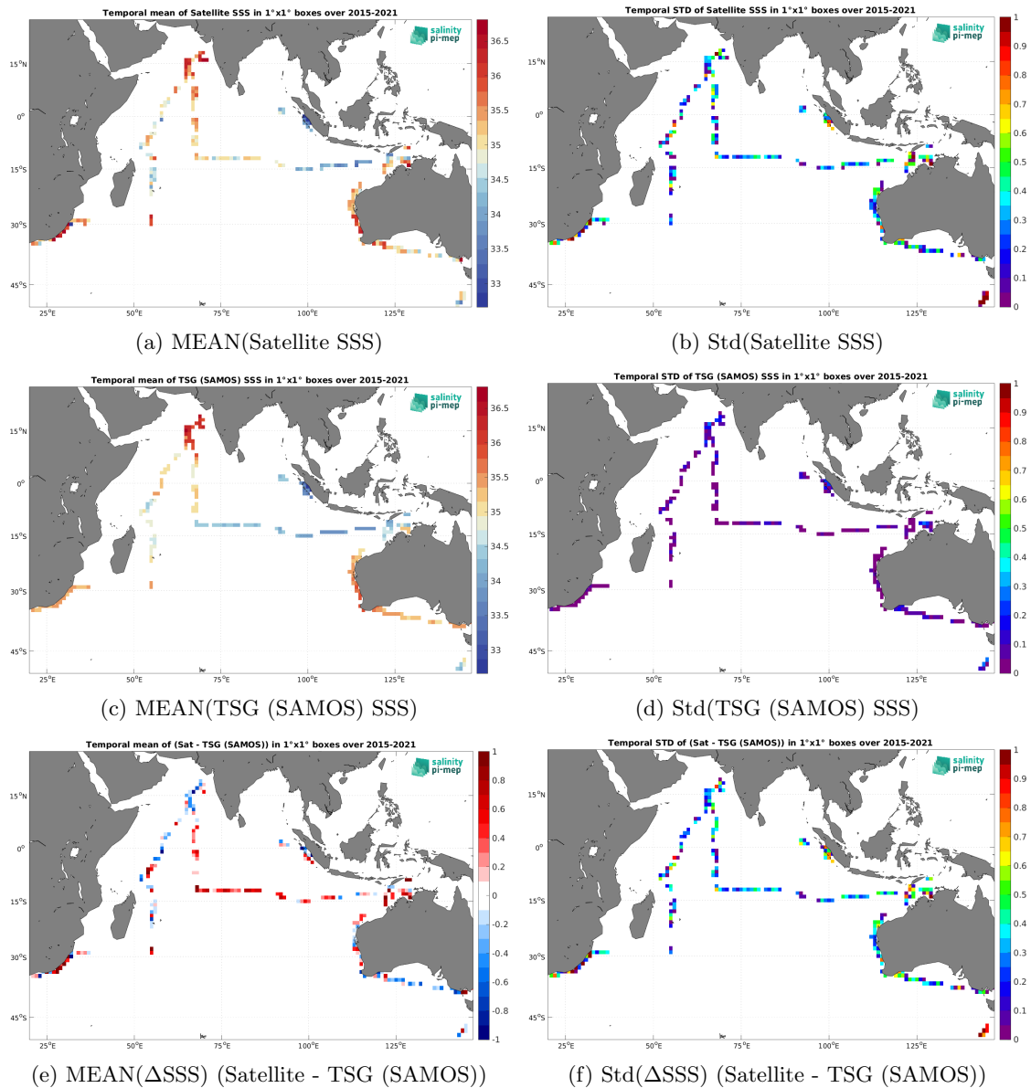
Figure 6: Temporal mean (left) and Std (right) of SSS from SMAP SSS L2 v5.0 (JPL) (top), TSG (SAMOS) (middle), and of \Delta SSS (Satellite - TSG (SAMOS)). Only match-up pairs are used to generate these maps.
