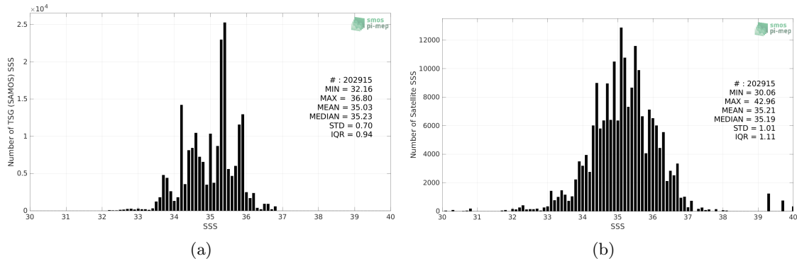
Figure 2: Histograms of SSS from TSG (SAMOS) (a) and SMAP SSS L2 v5.0 (JPL) (b) considering all match-up pairs per bins of 0.1 over the Indian Ocean Pi-MEP region and for the full satellite product period.
