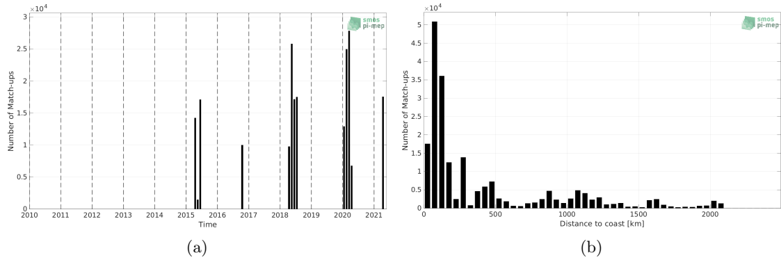
Figure 1: Number of match-ups between TSG (SAMOS) and SMAP SSS L2 v5.0 (JPL) SSS as a function of time (a) and as function of the distance to coast (b) over the Indian Ocean Pi-MEP region and for the full satellite product period.
