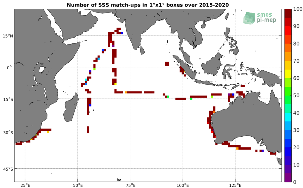
Figure 4: Number of SSS match-ups between TSG (SAMOS) SSS and the SMAP SSS L2 v5.0 (JPL) SSS product for the Indian Ocean Pi-MEP region over 1°x1° boxes and for the full satellite product period.
