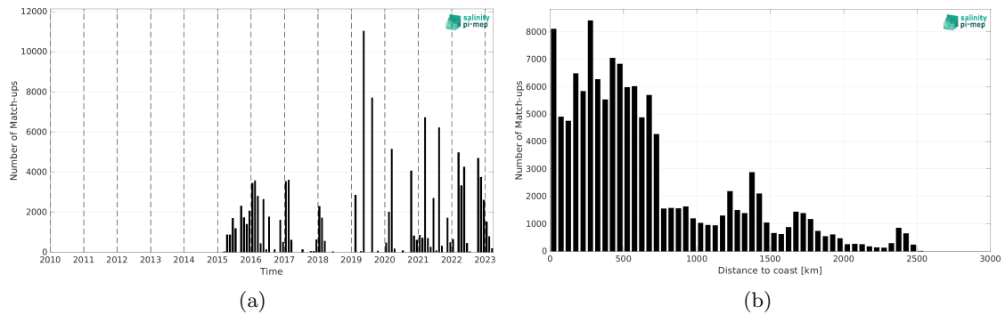
Figure 2: Number of match-ups between TSG (LEGOS-DM) and SMAP SSS L2 v5.0 (JPL) SSS as a function of time (a) and as function of the distance to coast (b) over the Indian Ocean Pi-MEP region and for the full satellite product period.
