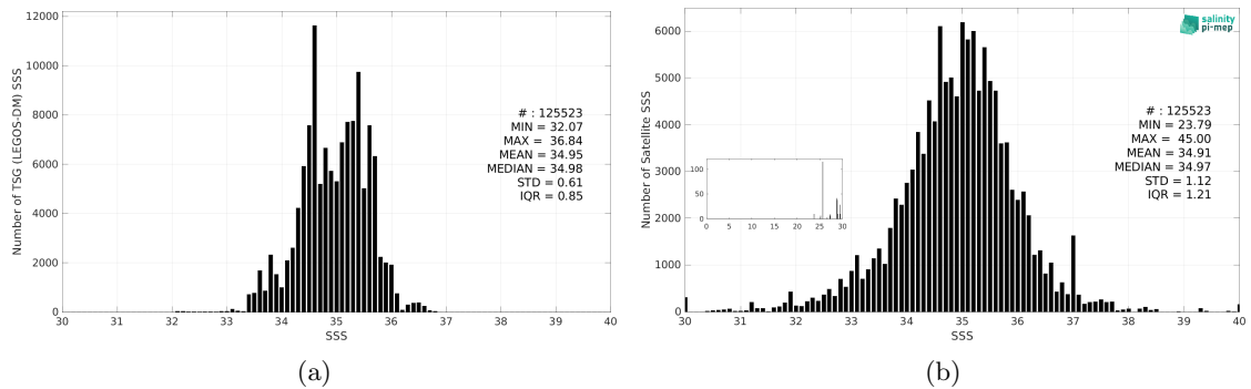
Figure 3: Histograms of SSS from TSG (LEGOS-DM) (a) and SMAP SSS L2 v5.0 (JPL) (b) considering all match-up pairs per bins of 0.1 over the Indian Ocean Pi-MEP region and for the full satellite product period.
