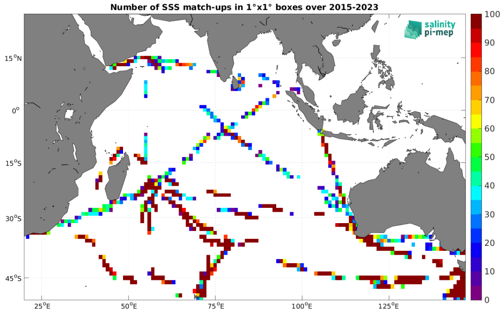
Figure 5: Number of SSS match-ups between TSG (LEGOS-DM) SSS and the SMAP SSS L2 v5.0 (JPL) SSS product for the Indian Ocean Pi-MEP region over 1^\circ \times 1^\circ boxes and for the full satellite product period.
