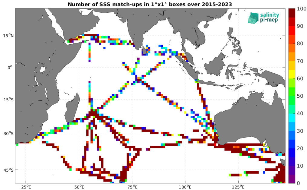
Figure 4: Number of SSS match-ups between TSG (LEGOS-DM) SSS and the SMAP SSS L2 v5.0 (JPL) SSS product for the Indian Ocean Pi-MEP region over 1^\circ \times 1^\circ boxes and for the full satellite product period.
