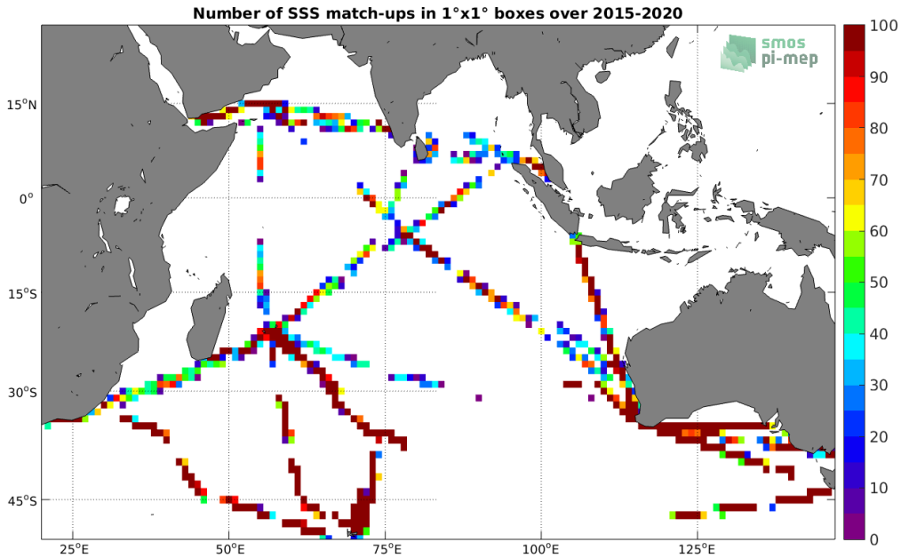
Figure 4: Number of SSS match-ups between TSG (LEGOS-DM) SSS and the SMAP SSS L2 v5.0 (JPL) SSS product for the Indian Ocean Pi-MEP region over 1°x1° boxes and for the full satellite product period.
