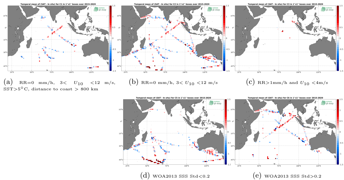
Figure 12: Temporal mean gridded over spatial boxes of size 1^\circ \times 1^\circ of \Delta SSS (SMAP SSS L2 v5.0 (JPL) - TSG (LEGOS-DM)) for 5 different subdatasets corresponding to:RR=0 mm/h, 3 < U_{10} < 12 m/s, SST >5^\circ\text{C} , distance to coast > 800 km (a), RR=0 mm/h, 3 < U_{10} < 12 m/s (b), RR >1 mm/h and U_{10} < 4 m/s (c), WOA2013 SSS Std <0.2 (d), WOA2013 SSS Std >0.2 (e).
