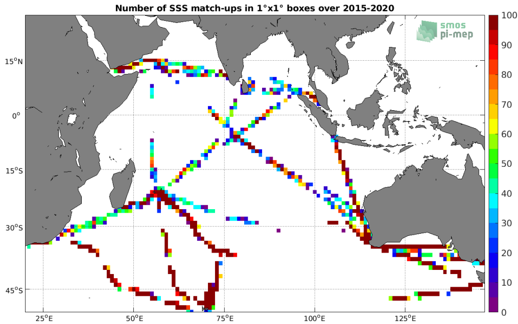
Figure 4: Number of SSS match-ups between TSG (LEGOS-DM) SSS and the SMAP SSS L2 v5.0 (JPL) SSS product for the Indian Ocean Pi-MEP region over 1°x1° boxes and for the full satellite product period.
