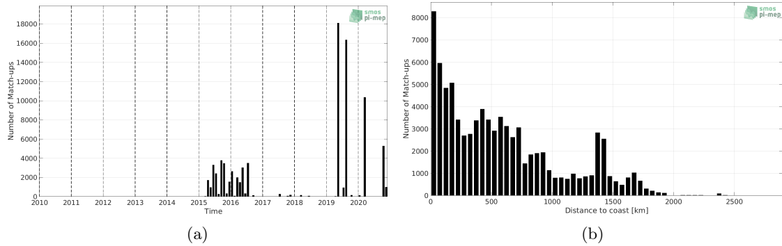
Figure 1: Number of match-ups between TSG (LEGOS-DM) and SMAP SSS L2 v5.0 (JPL) SSS as a function of time (a) and as function of the distance to coast (b) over the Indian Ocean Pi-MEP region and for the full satellite product period.
