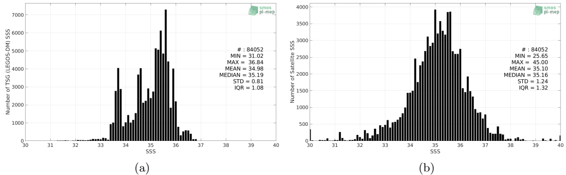
Figure 2: Histograms of SSS from TSG (LEGOS-DM) (a) and SMAP SSS L2 v5.0 (JPL) (b) considering all match-up pairs per bins of 0.1 over the Indian Ocean Pi-MEP region and for the full satellite product period.
