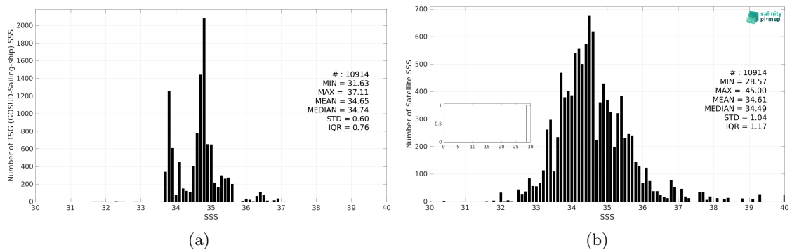
Figure 3: Histograms of SSS from TSG (GOSUD-Sailing-ship) (a) and SMAP SSS L2 v5.0 (JPL) (b) considering all match-up pairs per bins of 0.1 over the Indian Ocean Pi-MEP region and for the full satellite product period.
