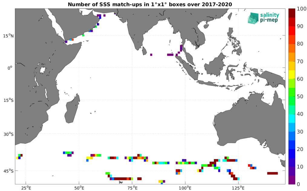
Figure 5: Number of SSS match-ups between TSG (GOSUD-Sailing-ship) SSS and the SMAP SSS L2 v5.0 (JPL) SSS product for the Indian Ocean Pi-MEP region over 1^\circ \times 1^\circ boxes and for the full satellite product period.
