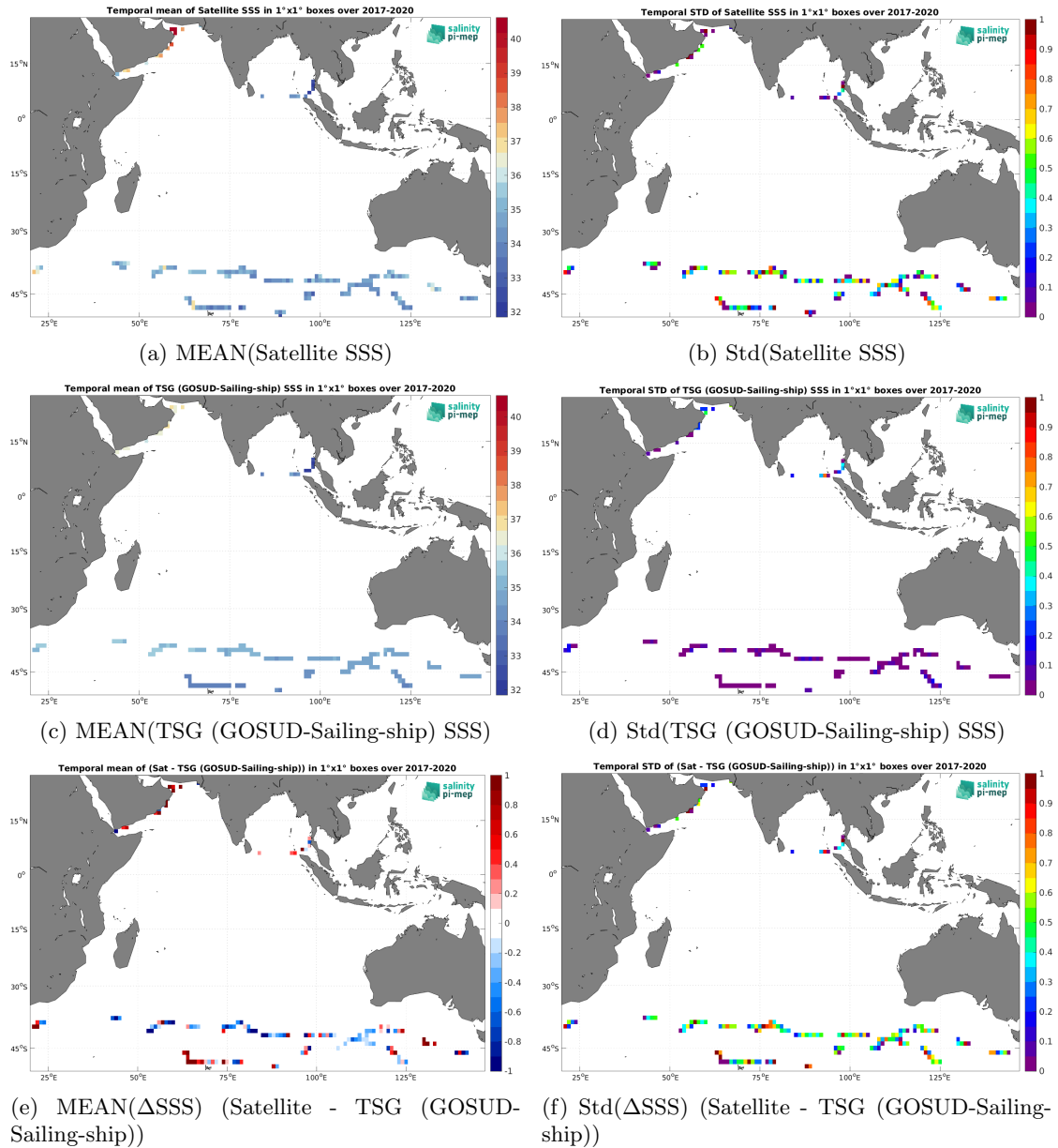
Figure 7: Temporal mean (left) and Std (right) of SSS from SMAP SSS L2 v5.0 (JPL) (top), TSG (GOSUD-Sailing-ship) (middle), and of \Delta SSS (Satellite - TSG (GOSUD-Sailing-ship)). Only match-up pairs are used to generate these maps.
