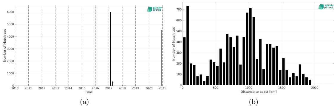
Figure 2: Number of match-ups between TSG (GOSUD-Sailing-ship) and SMAP SSS L2 v5.0 (JPL) SSS as a function of time (a) and as function of the distance to coast (b) over the Indian Ocean Pi-MEP region and for the full satellite product period.
