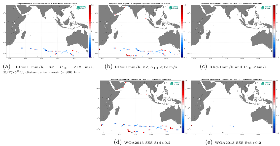
Figure 14: Temporal mean gridded over spatial boxes of size 1^\circ \times 1^\circ of \Delta\text{SSS} (SMAP SSS L2 v5.0 (JPL) - TSG (GOSUD-Sailing-ship)) for 5 different subdatasets corresponding to:RR=0 mm/h, 3 < U_{10} < 12 m/s, SST > 5^\circ\text{C} , distance to coast > 800 km (a), RR=0 mm/h, 3 < U_{10} < 12 m/s (b), RR > 1 mm/h and U_{10} < 4 m/s (c), WOA2013 SSS Std < 0.2 (d), WOA2013 SSS Std > 0.2 (e).
