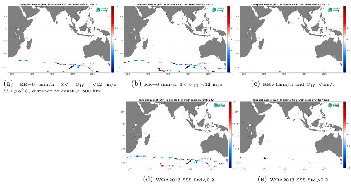
Figure 12: Temporal mean gridded over spatial boxes of size 1^\circ \times 1^\circ of \Delta\text{SSS} (SMAP SSS L2 v5.0 (JPL) - TSG (GOSUD-Sailing-ship)) for 5 different subdatasets corresponding to:RR=0 mm/h, 3 < U_{10} < 12 m/s, SST > 5°C, distance to coast > 800 km (a), RR=0 mm/h, 3 < U_{10} < 12 m/s (b), RR > 1mm/h and U_{10} < 4 m/s (c), WOA2013 SSS Std < 0.2 (d), WOA2013 SSS Std > 0.2 (e).
