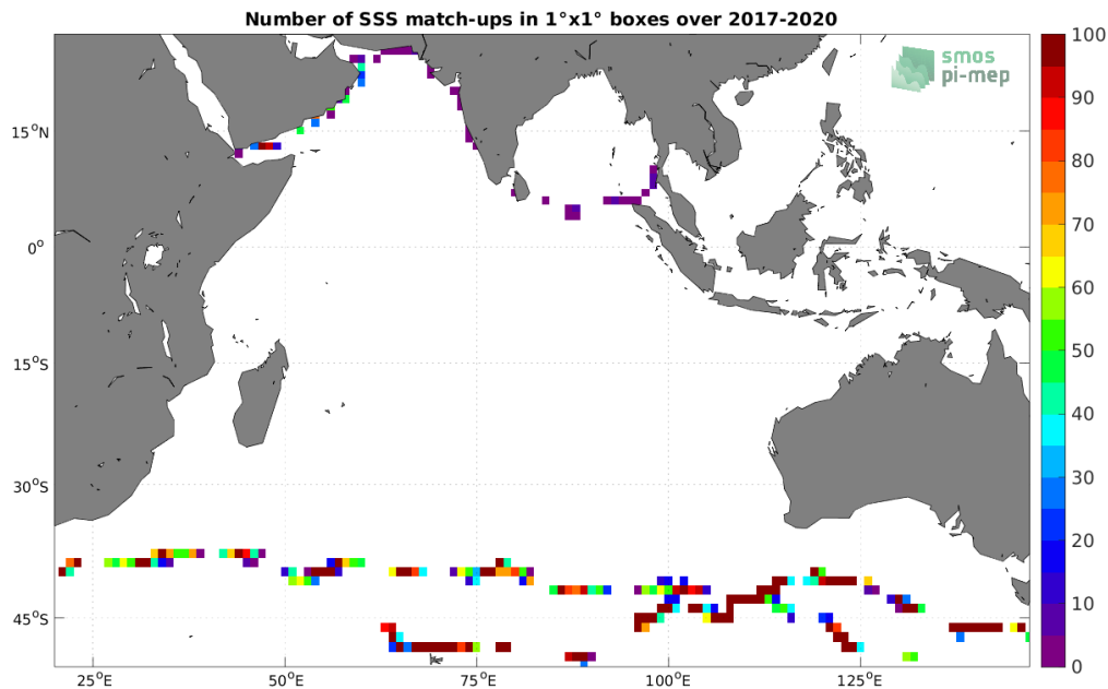
Figure 4: Number of SSS match-ups between TSG (GOSUD-Sailing-ship) SSS and the SMAP SSS L2 v5.0 (JPL) SSS product for the Indian Ocean Pi-MEP region over 1^{\circ} \times 1^{\circ} boxes and for the full satellite product period.
