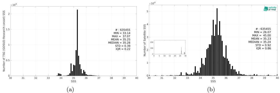
Figure 3: Histograms of SSS from TSG (GOSUD-Research-vessel) (a) and SMAP SSS L2 v5.0 (JPL) (b) considering all match-up pairs per bins of 0.1 over the Indian Ocean Pi-MEP region and for the full satellite product period.
