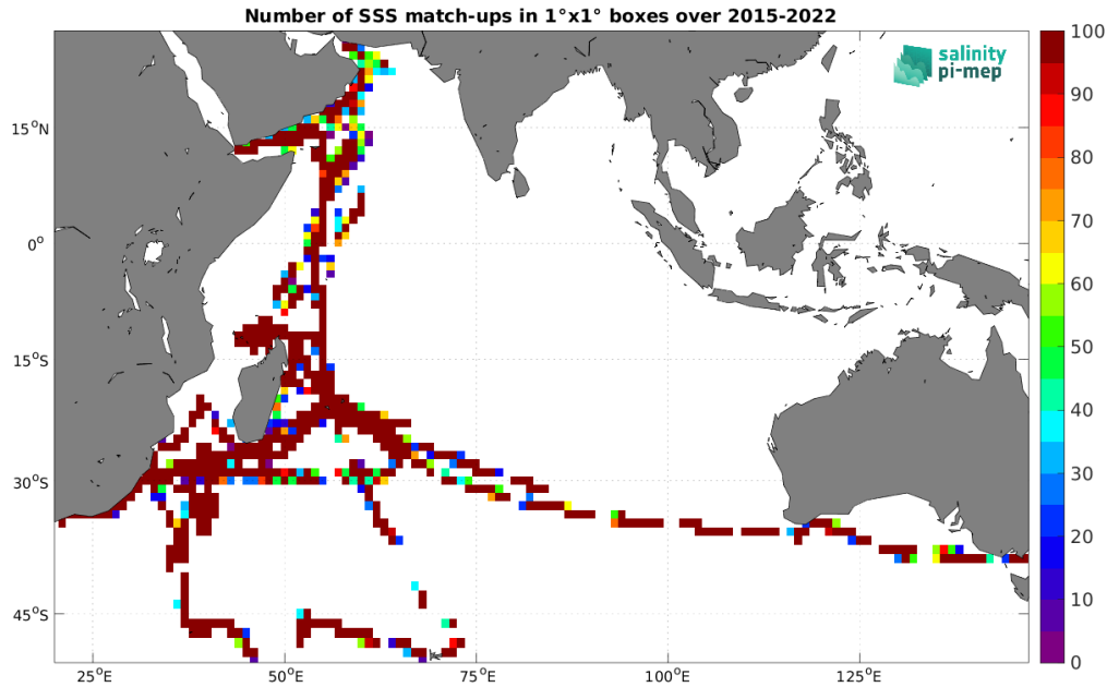
Figure 5: Number of SSS match-ups between TSG (GOSUD-Research-vessel) SSS and the SMAP SSS L2 v5.0 (JPL) SSS product for the Indian Ocean Pi-MEP region over 1^\circ \times 1^\circ boxes and for the full satellite product period.
