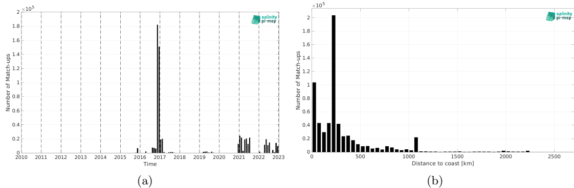
Figure 2: Number of match-ups between TSG (GOSUD-Research-vessel) and SMAP SSS L2 v5.0 (JPL) SSS as a function of time (a) and as function of the distance to coast (b) over the Indian Ocean Pi-MEP region and for the full satellite product period.
